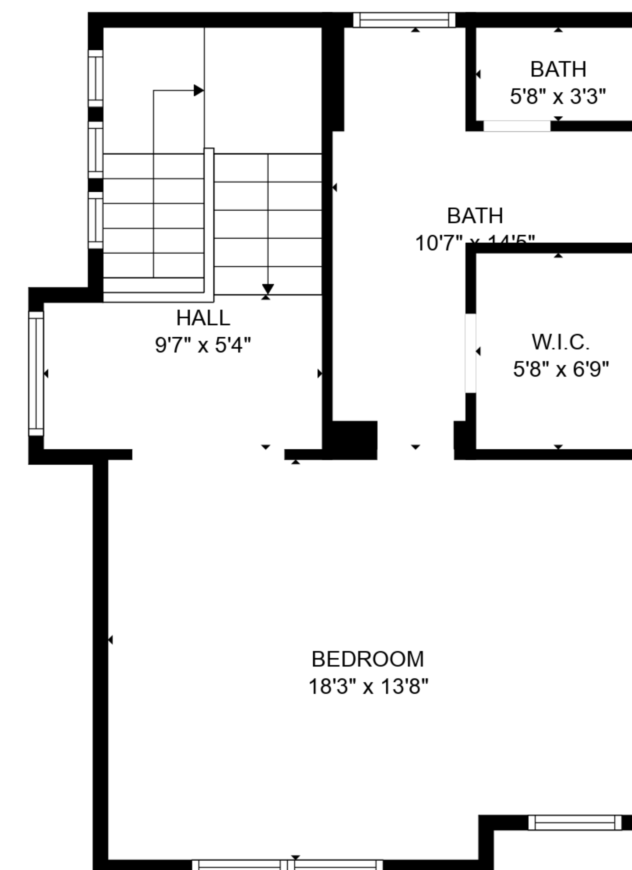
FLOOR 2
