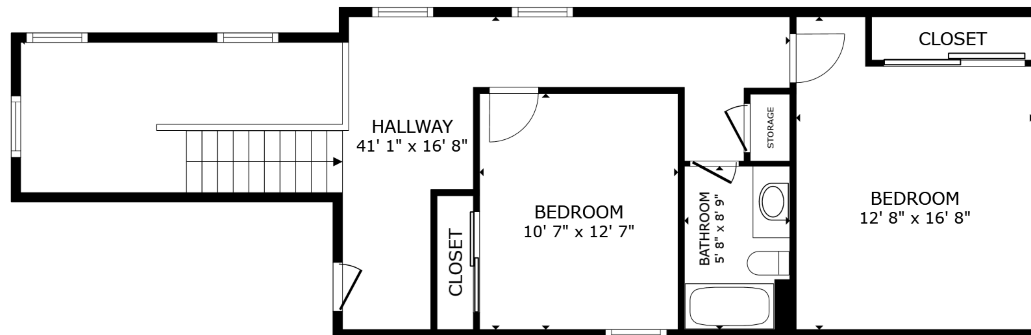
FLOOR 2
