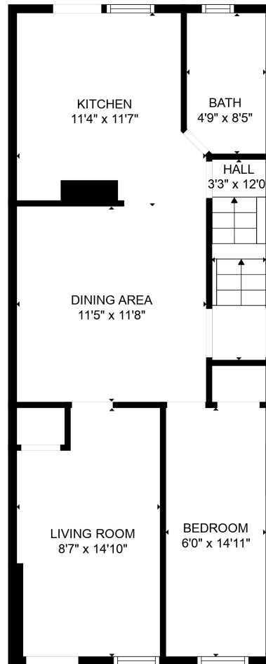
FLOOR 2
