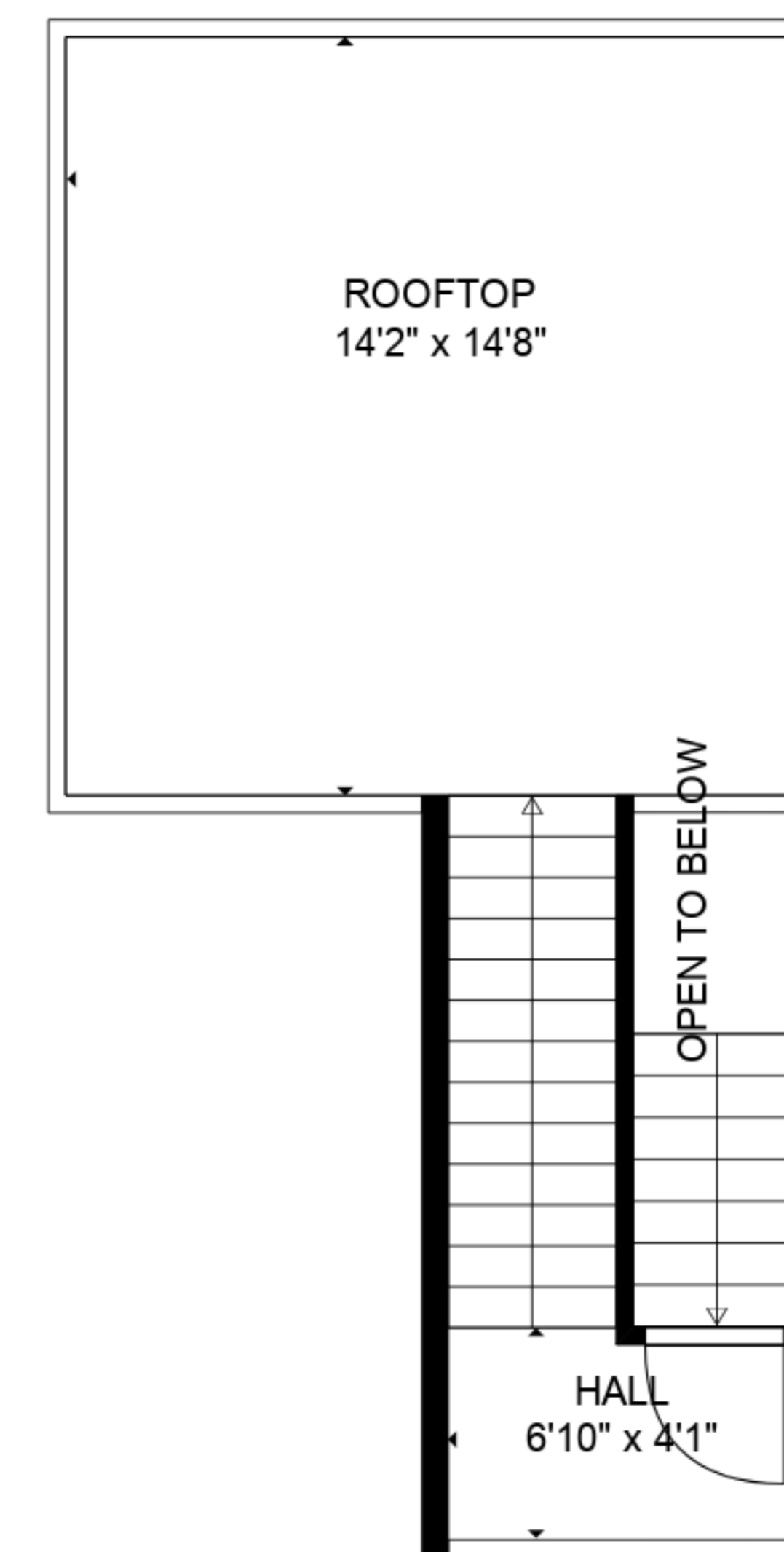
FLOOR 4
