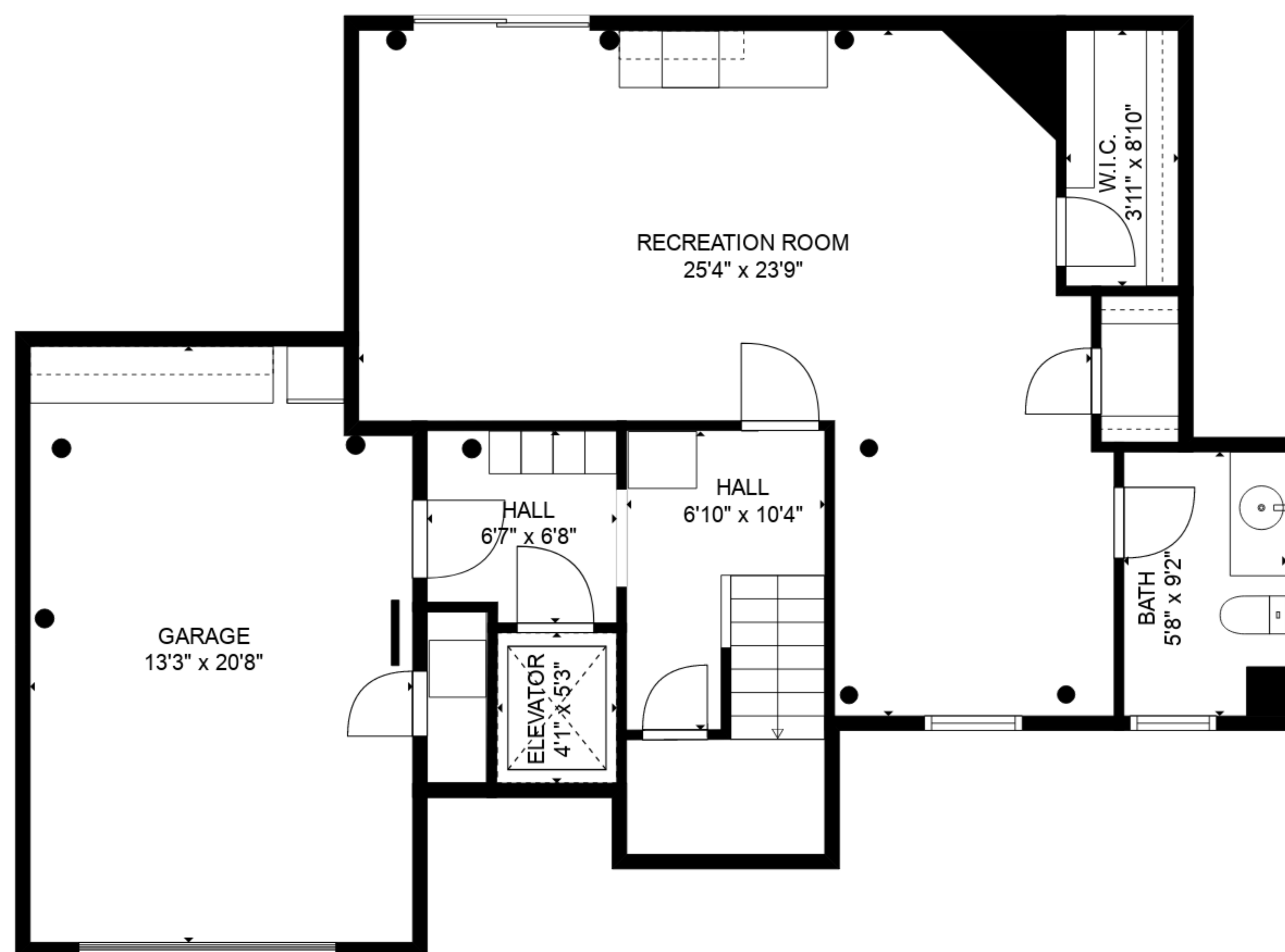
FLOOR 1
