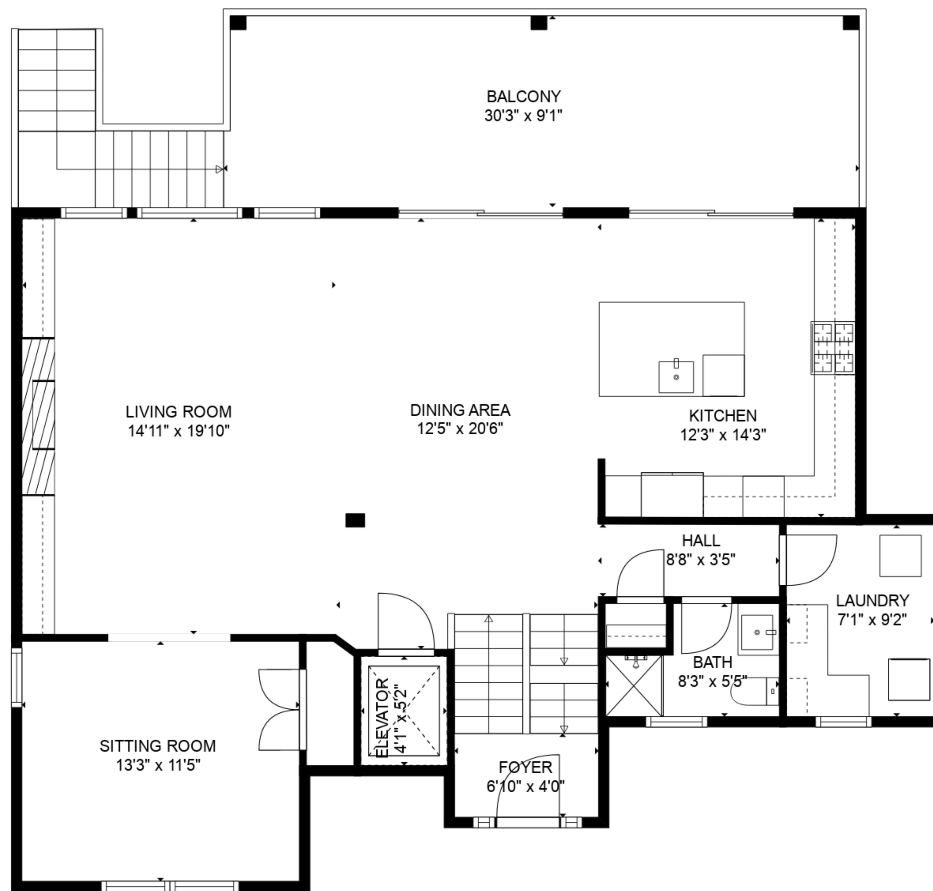
FLOOR 2
