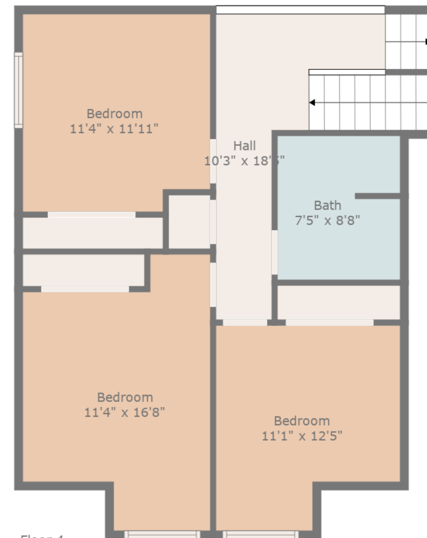
Floor 4
