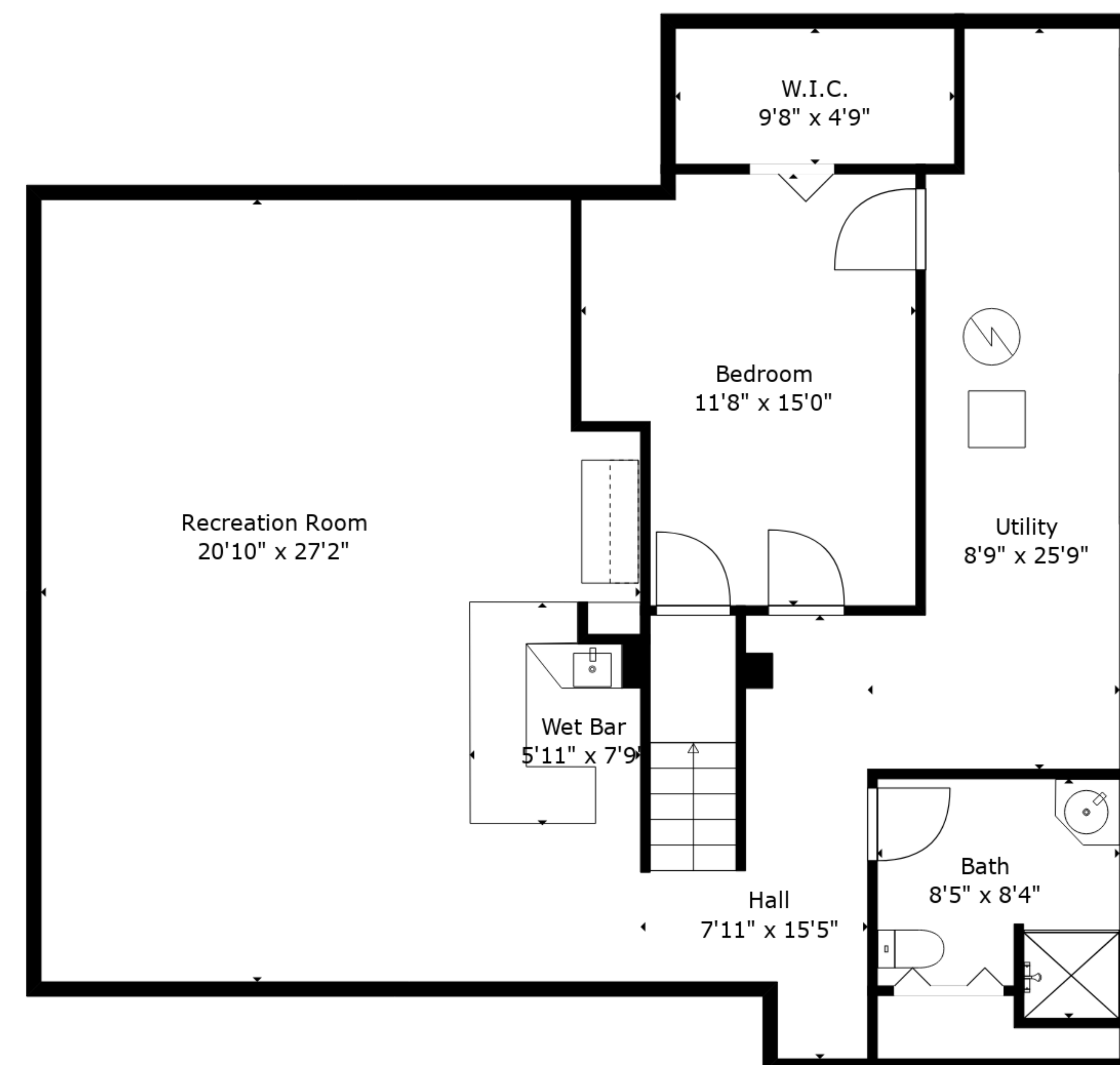
Floor 1
