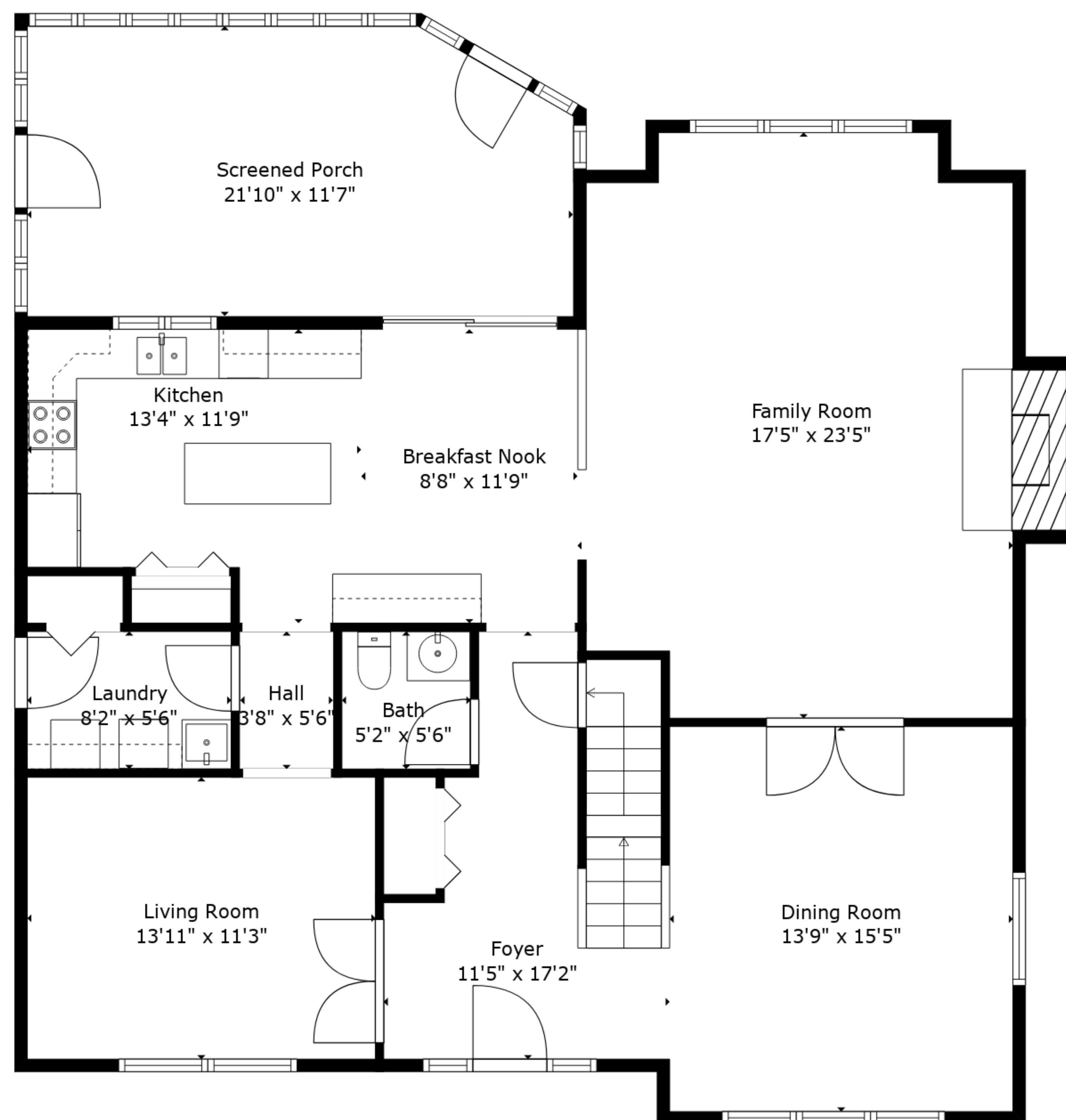
Floor 2
