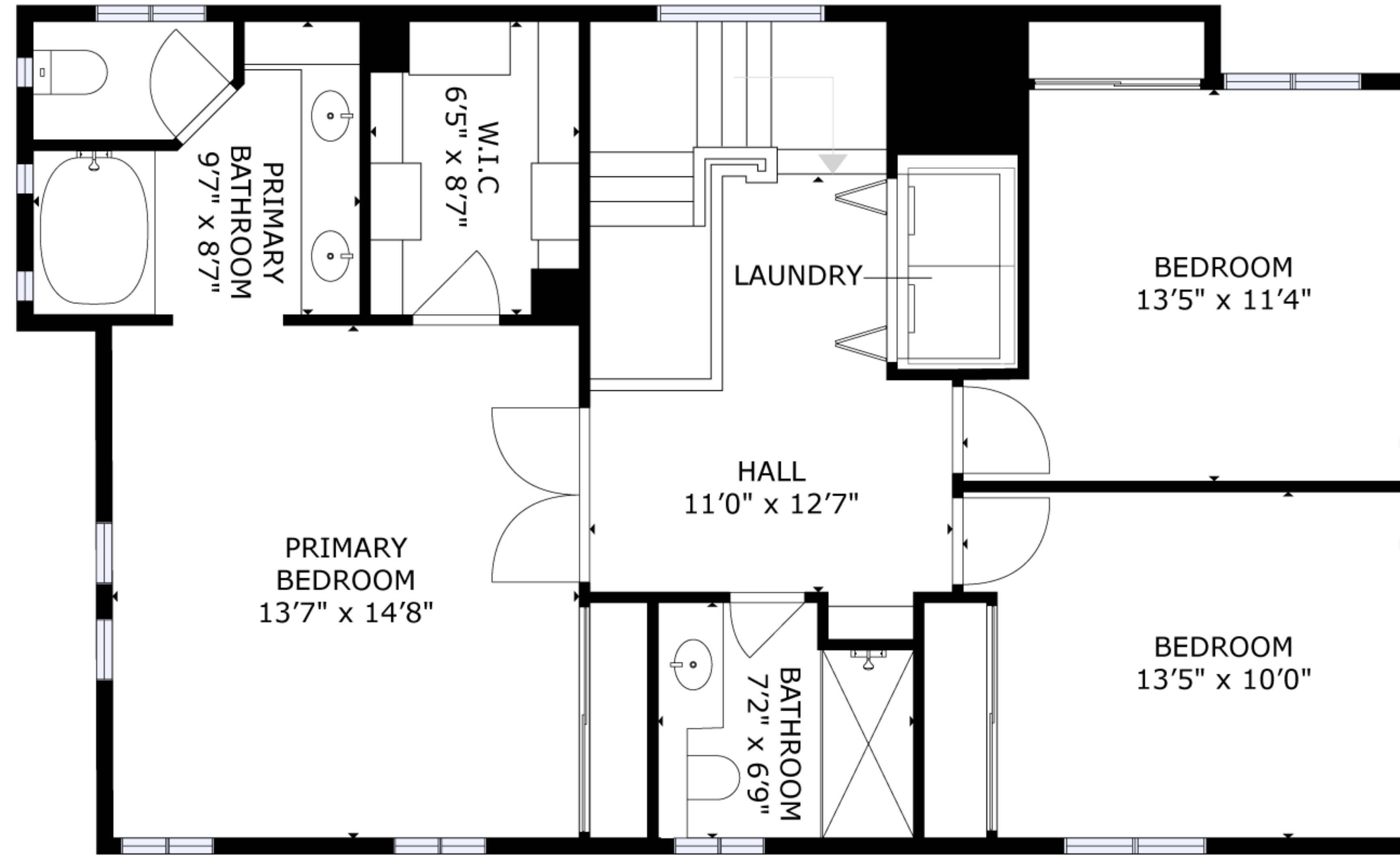
FLOOR 2
