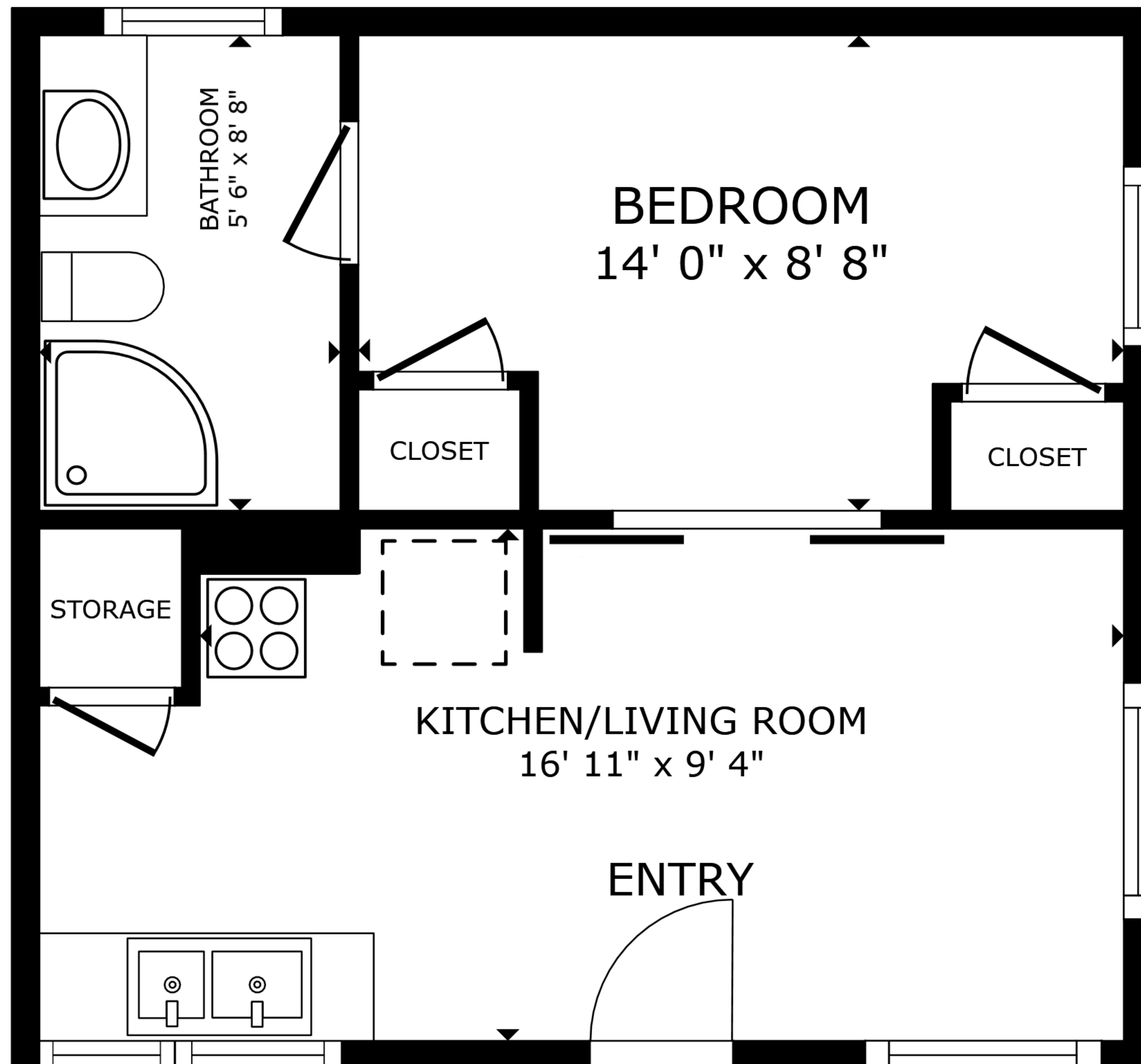
FLOOR PLAN
