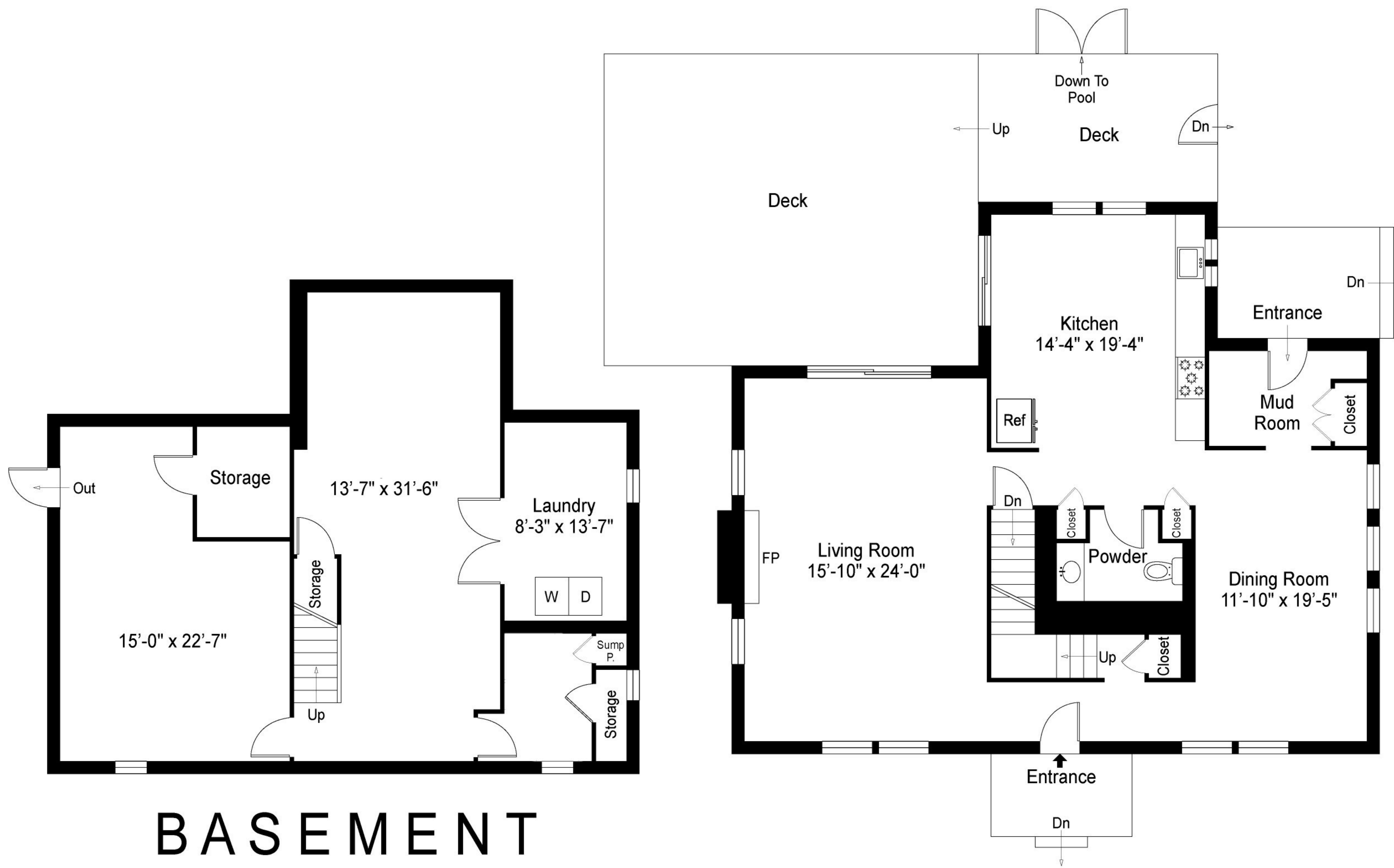
FIRST FLOOR
