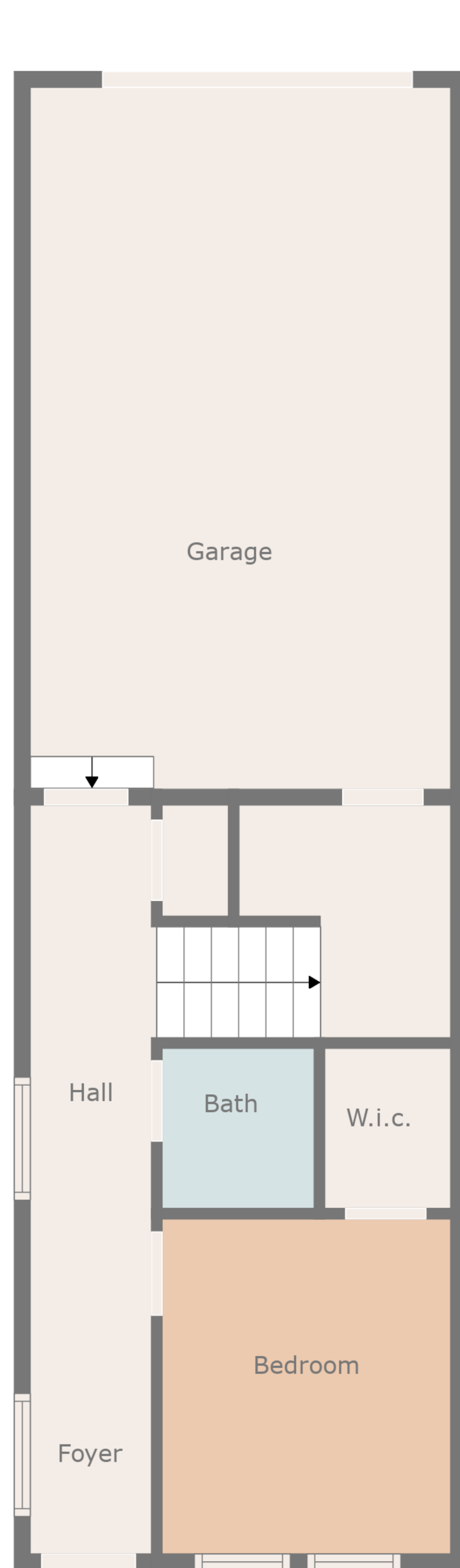
Floor 1
