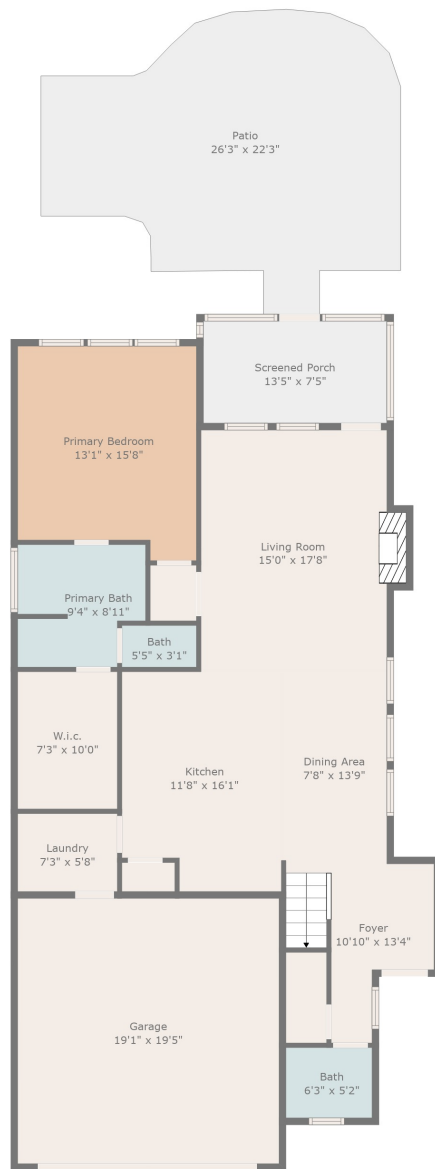
Floor 1
