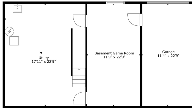
Floor 1
