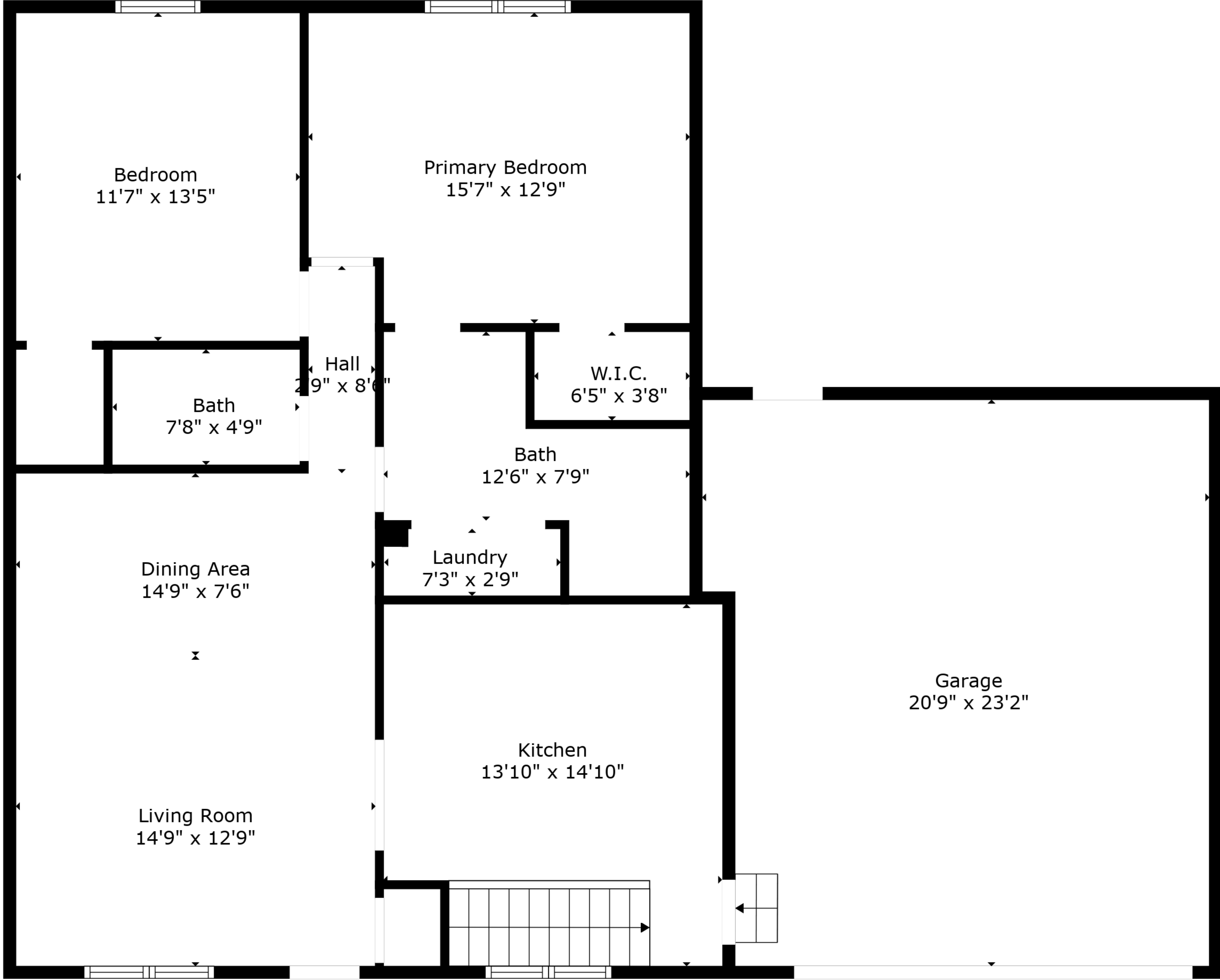
Floor 2
