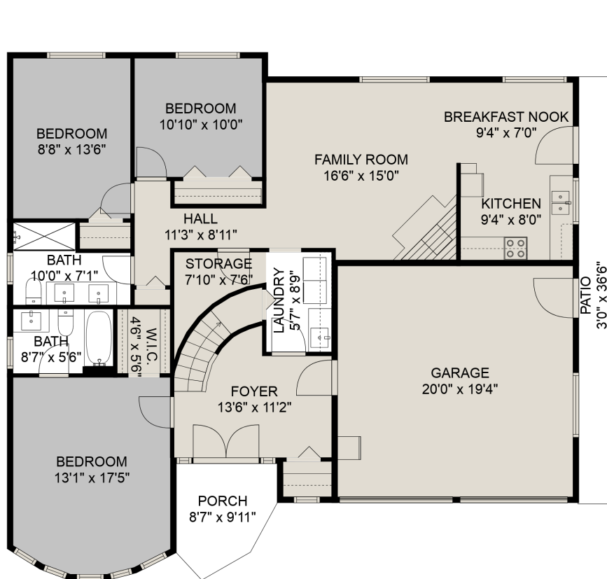
FLOOR 1
