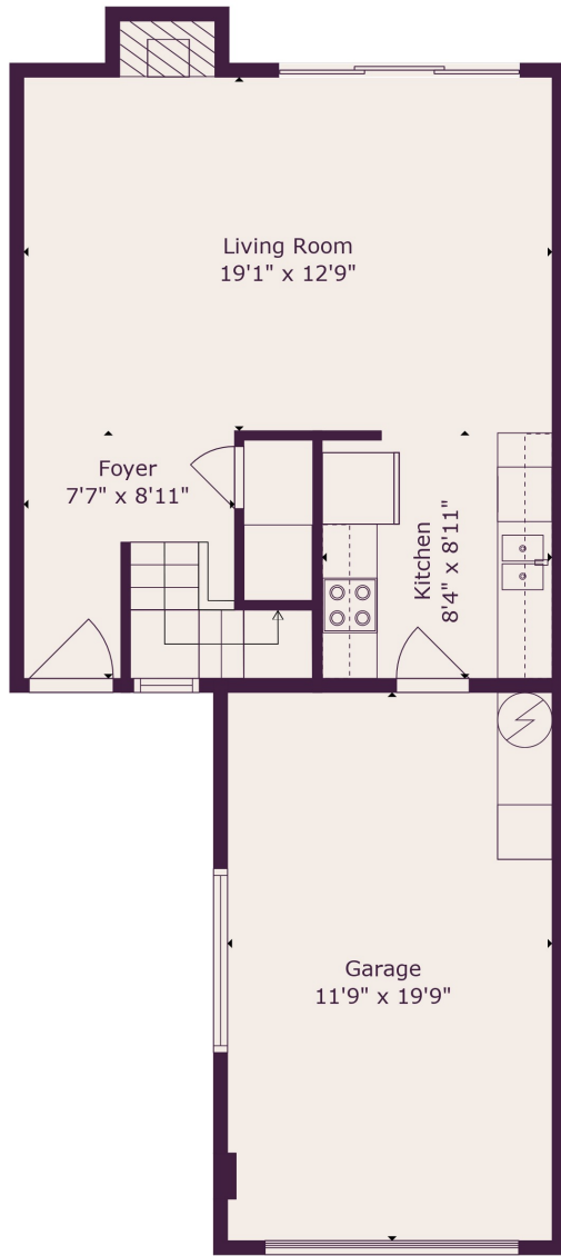
Floor 1
