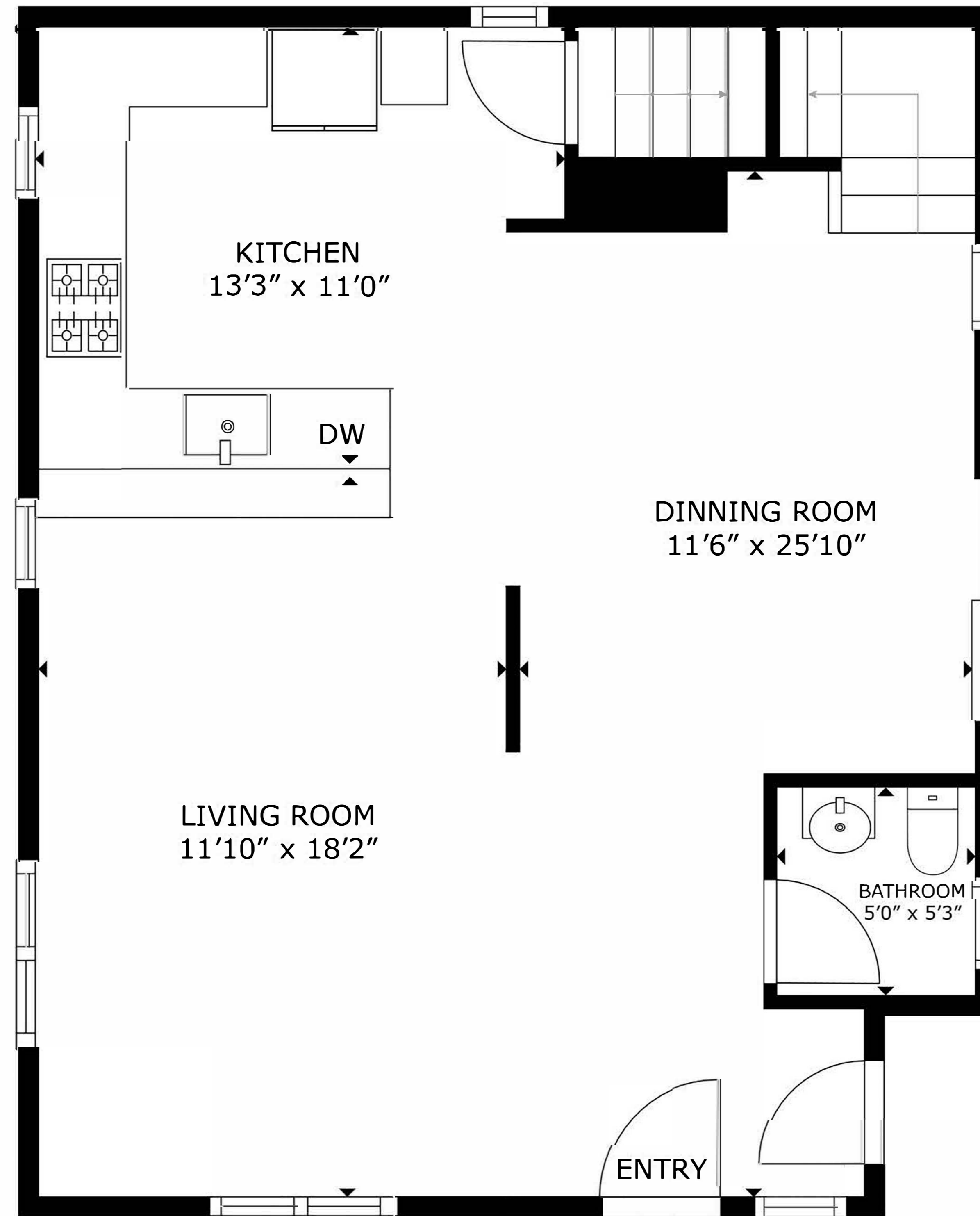
FLOOR 1
