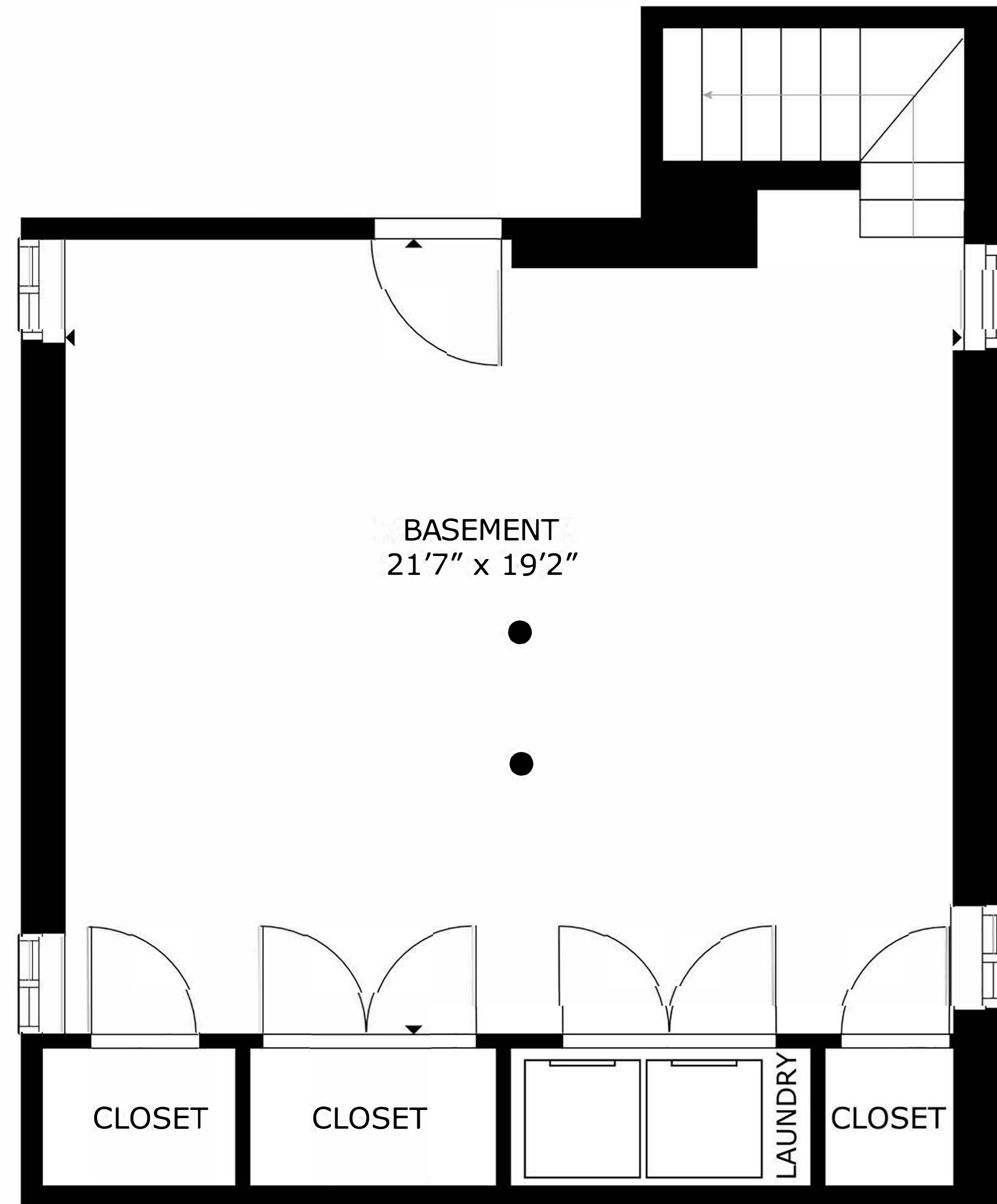
BASEMENT
