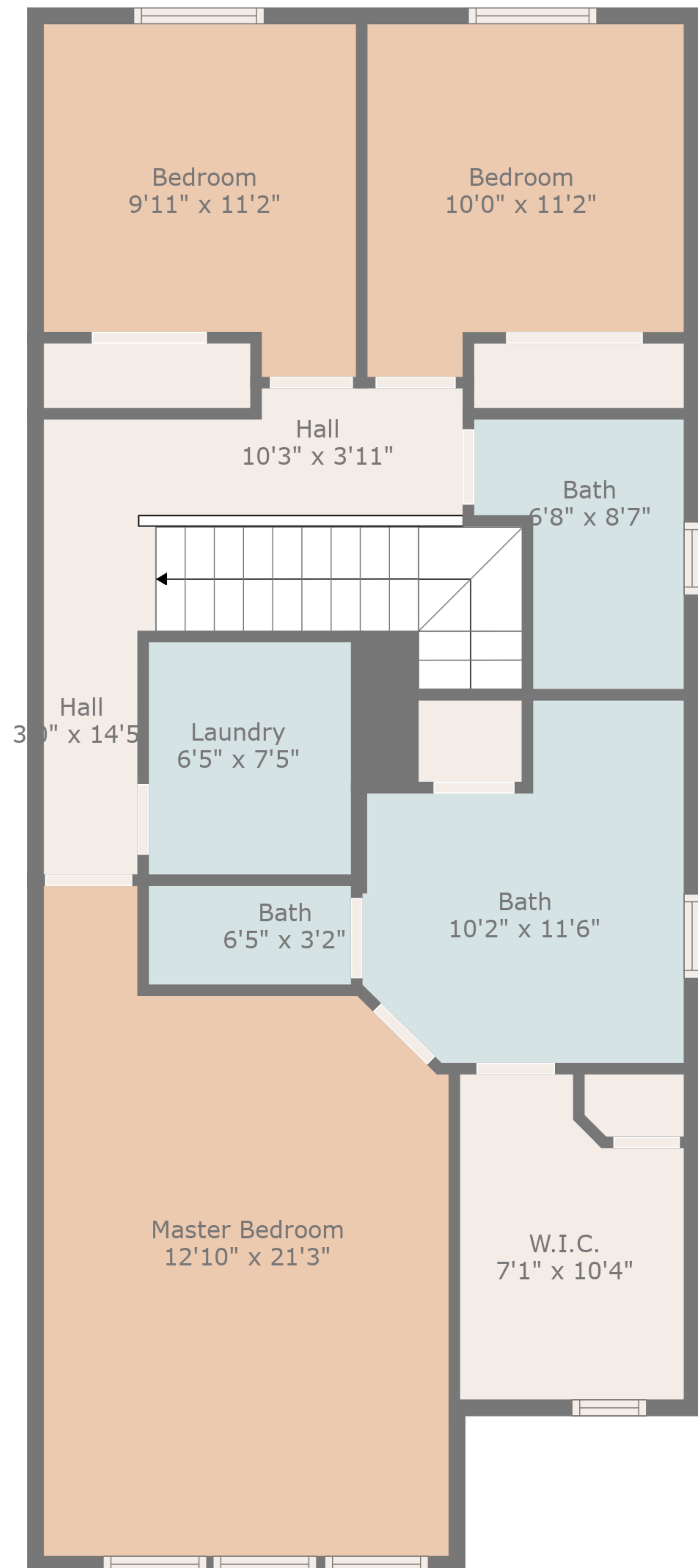
Floor 3
