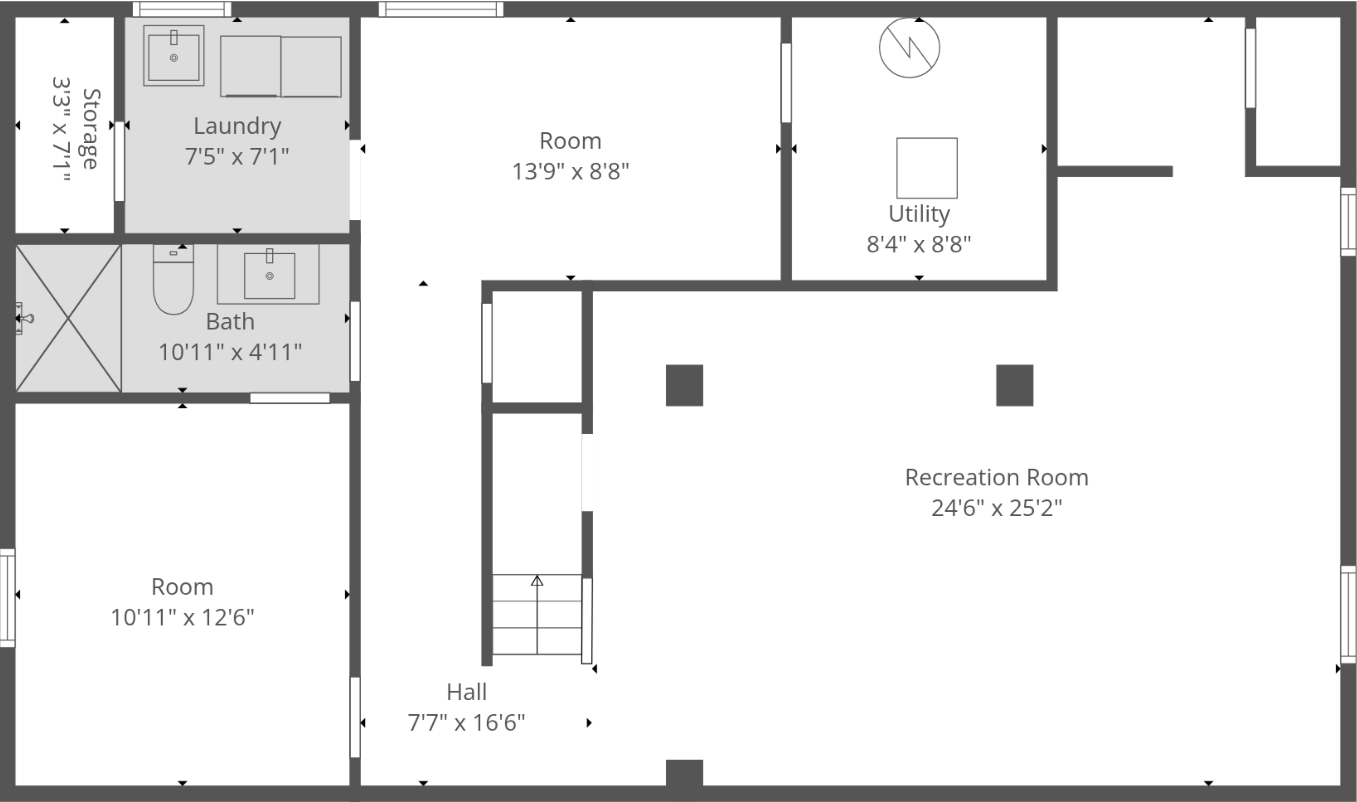
Floor 1
