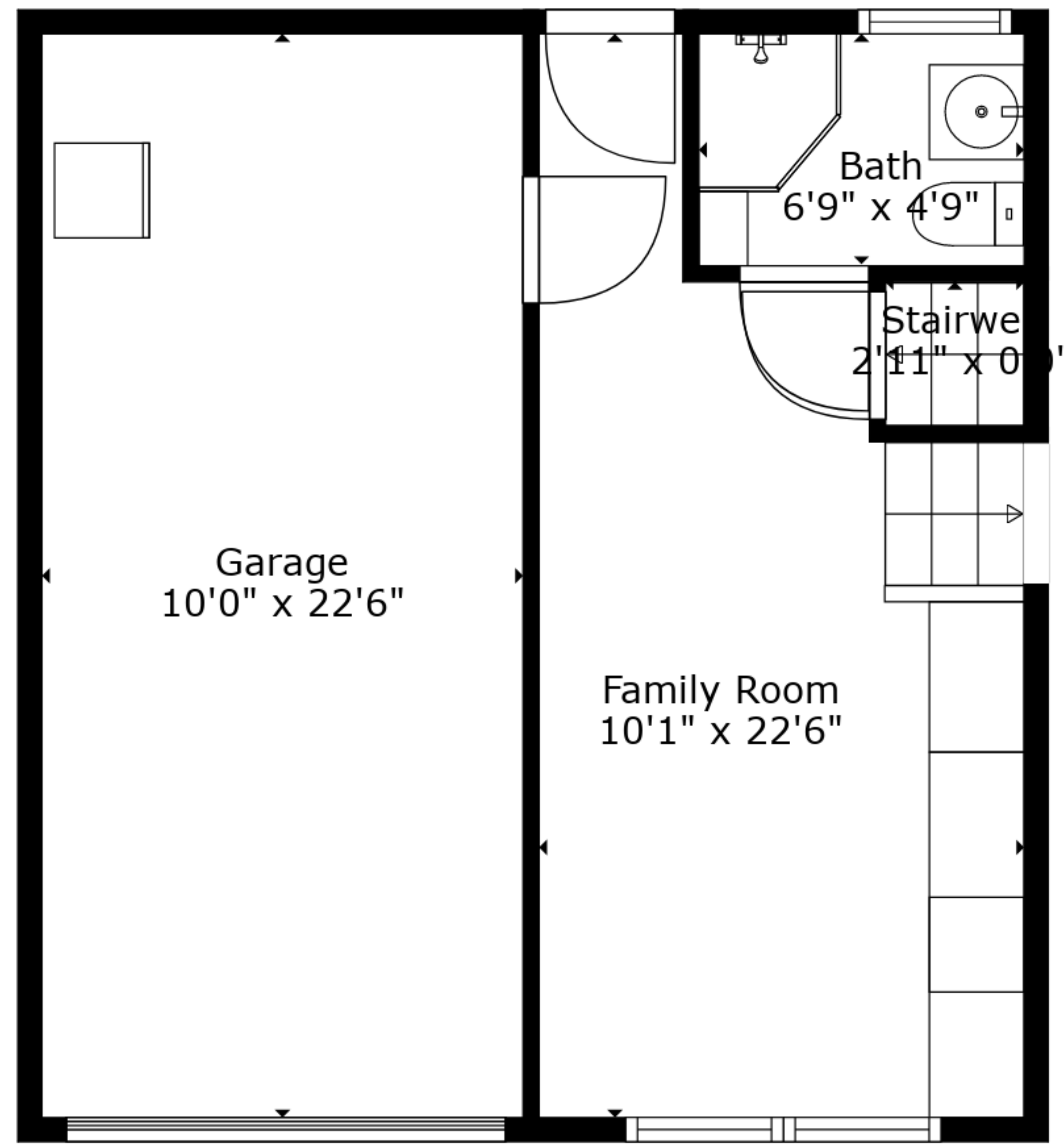
Floor 2
