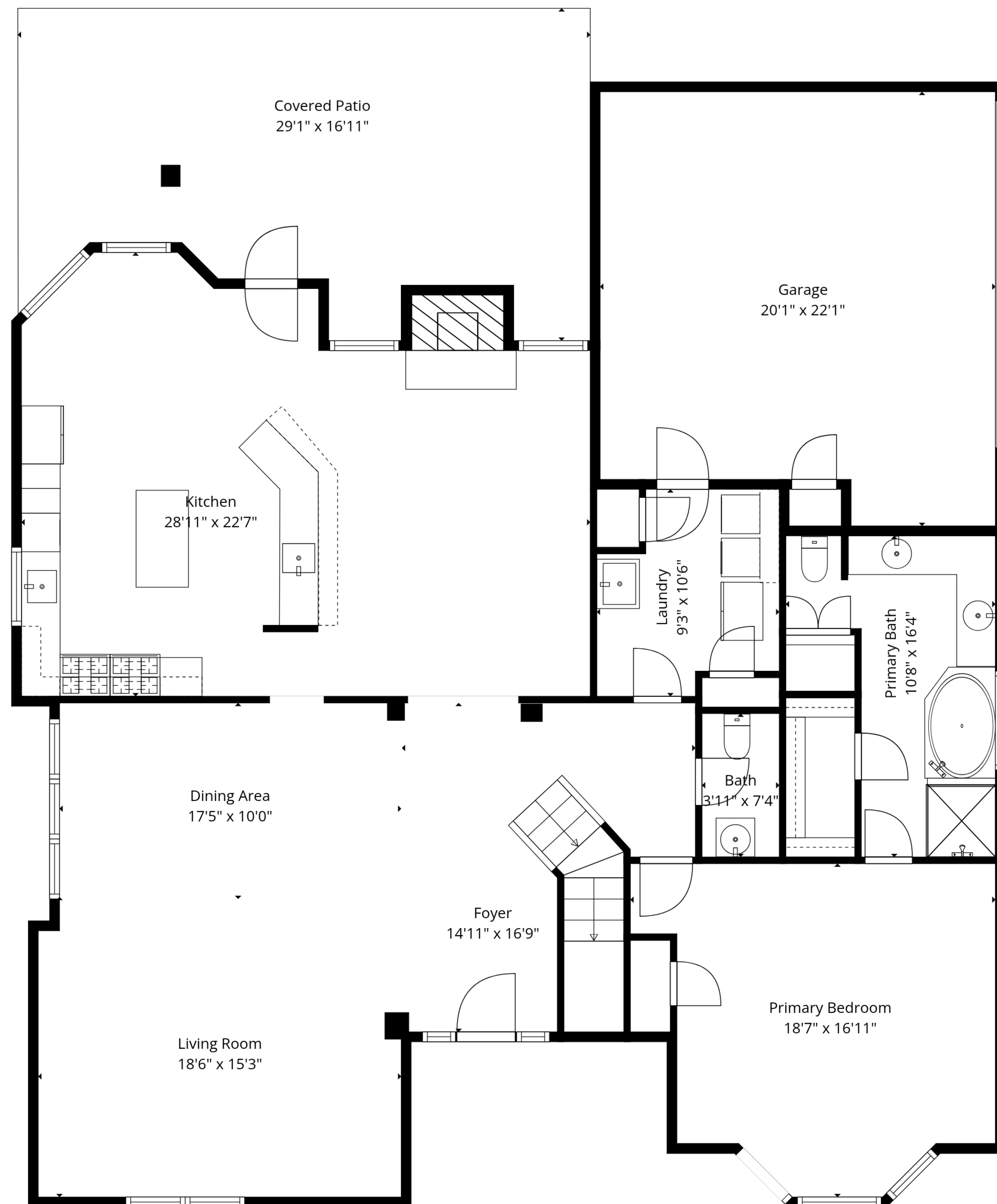
Floor 1
