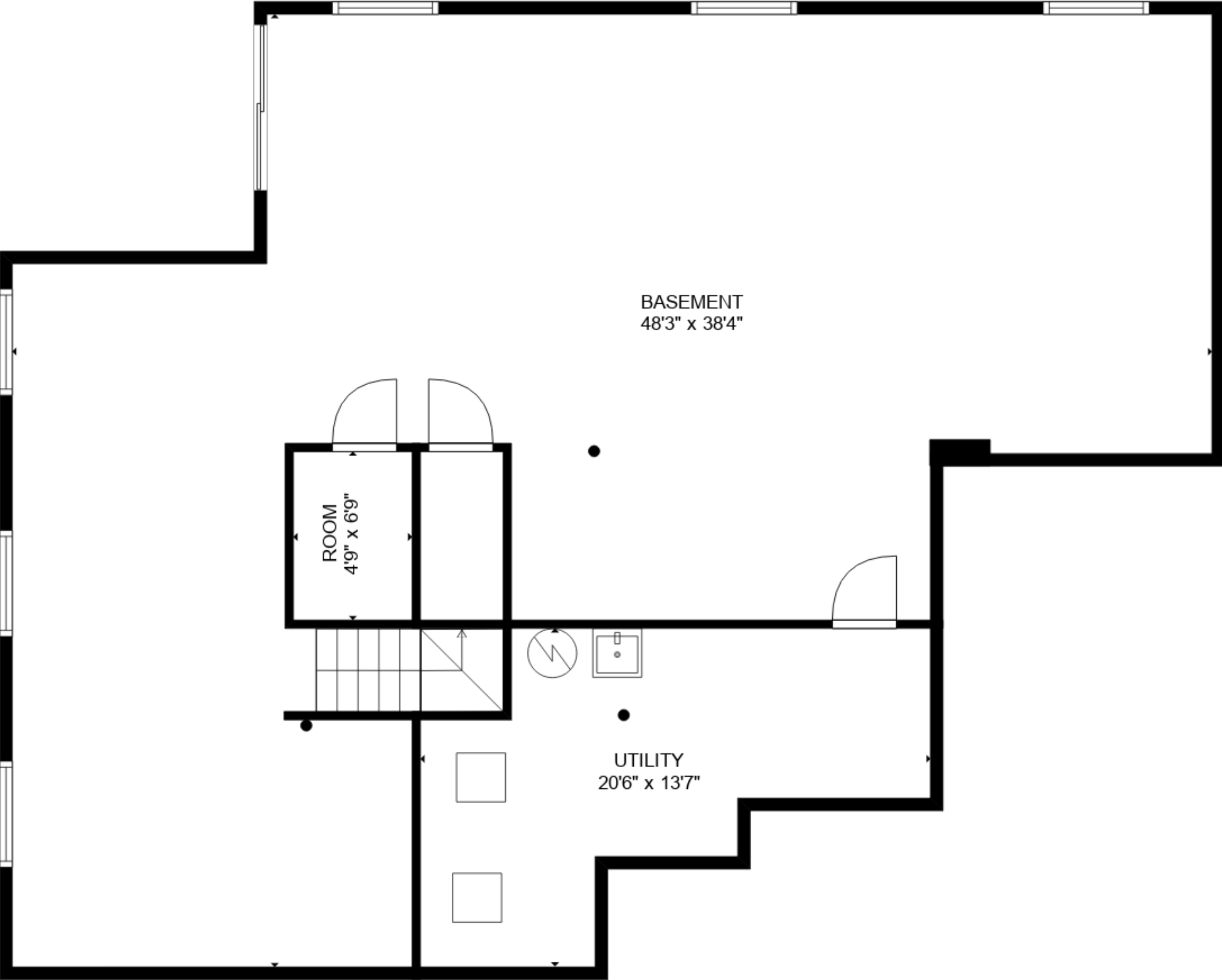
FLOOR 1
