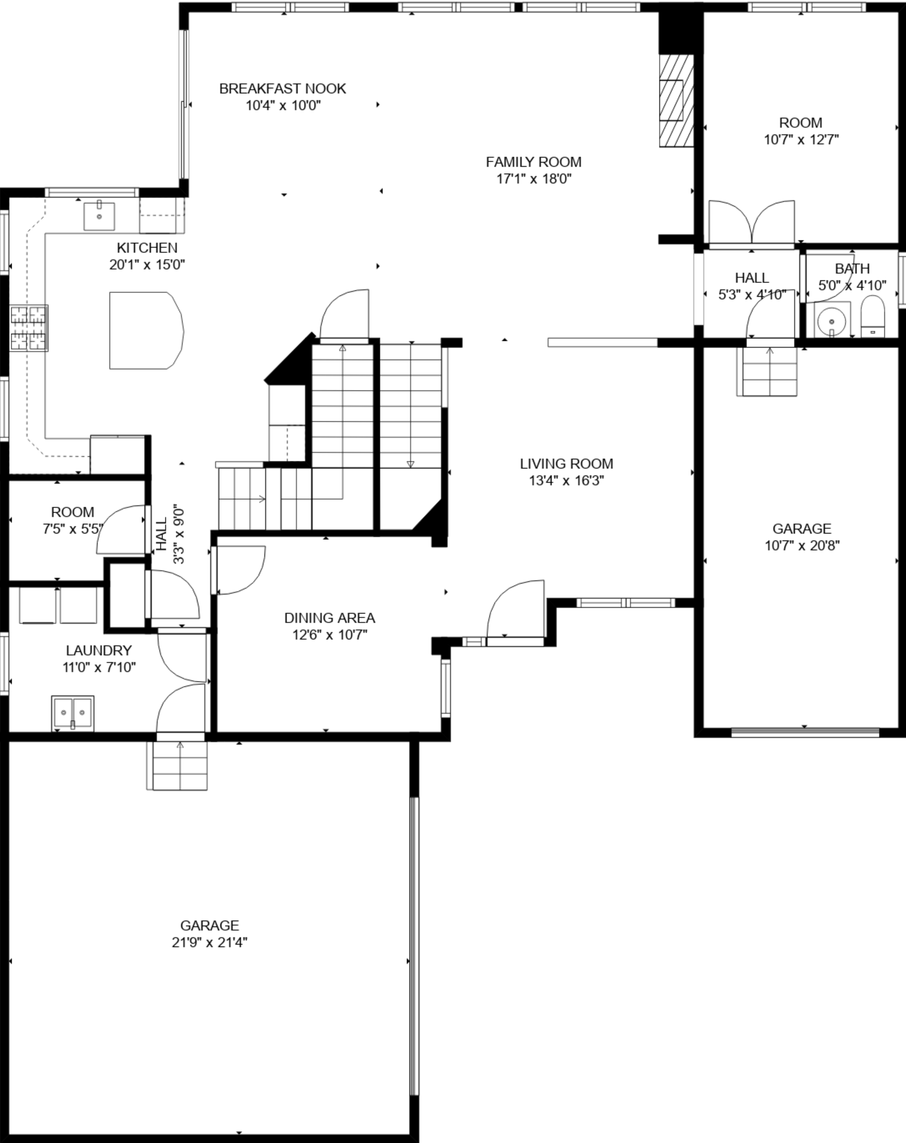
FLOOR 2
