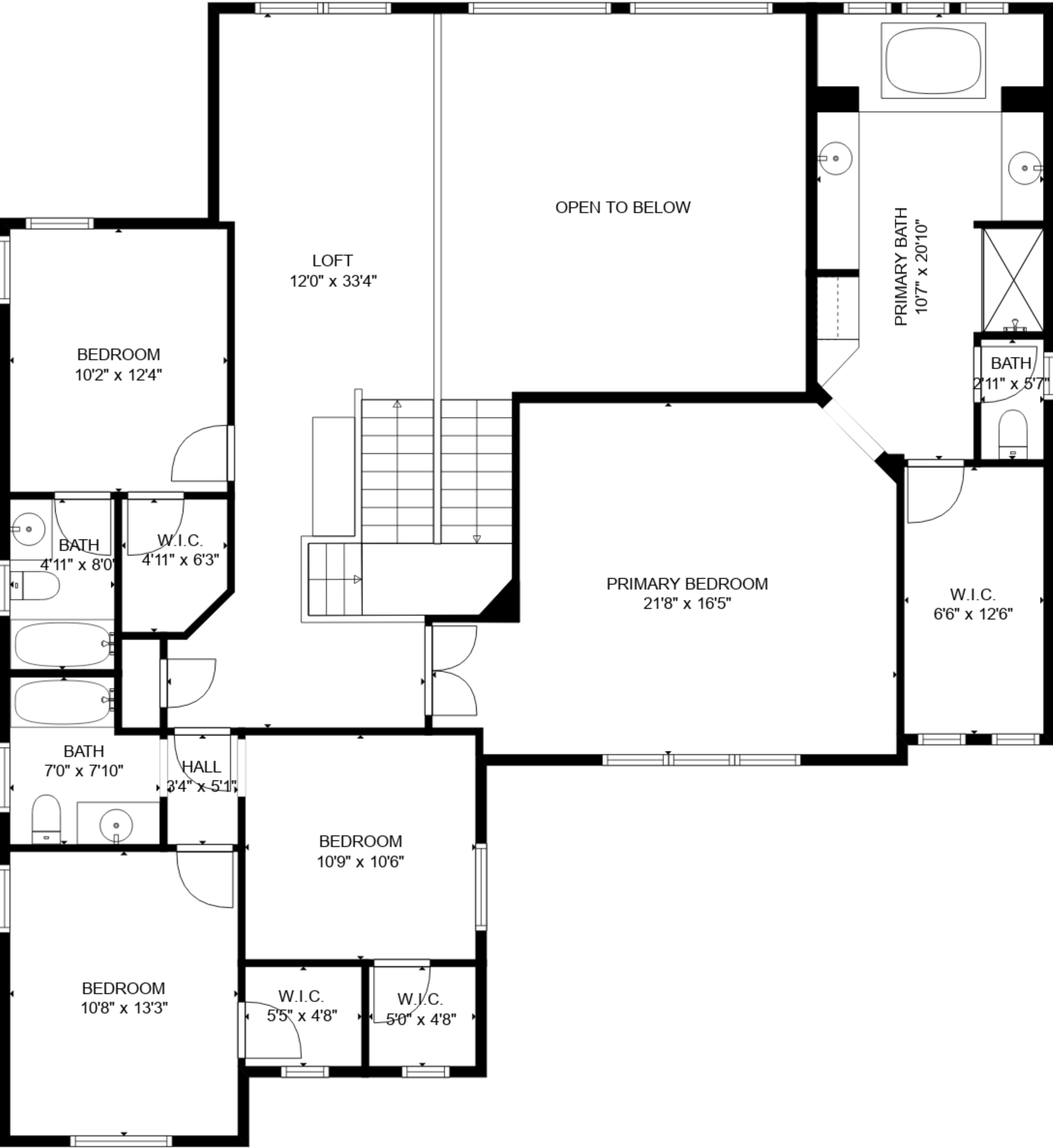
FLOOR 3
