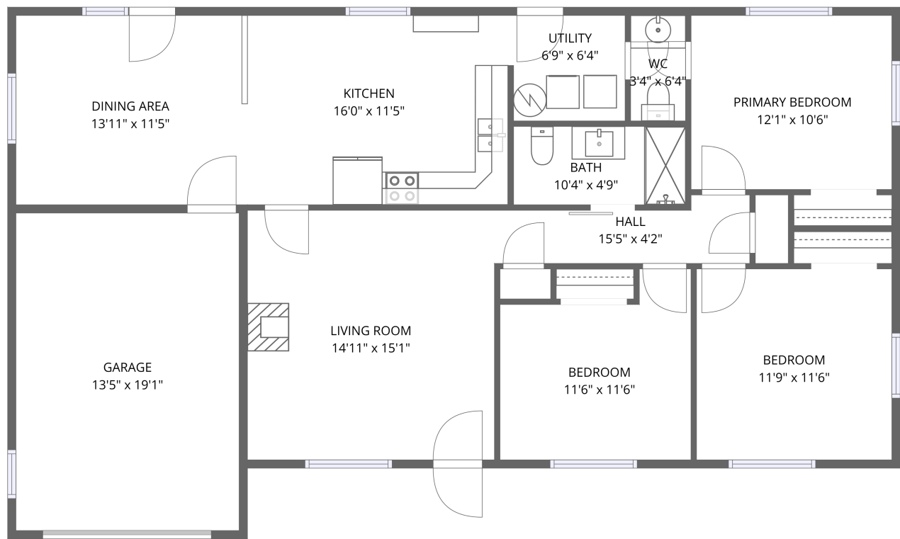
FLOOR 1
