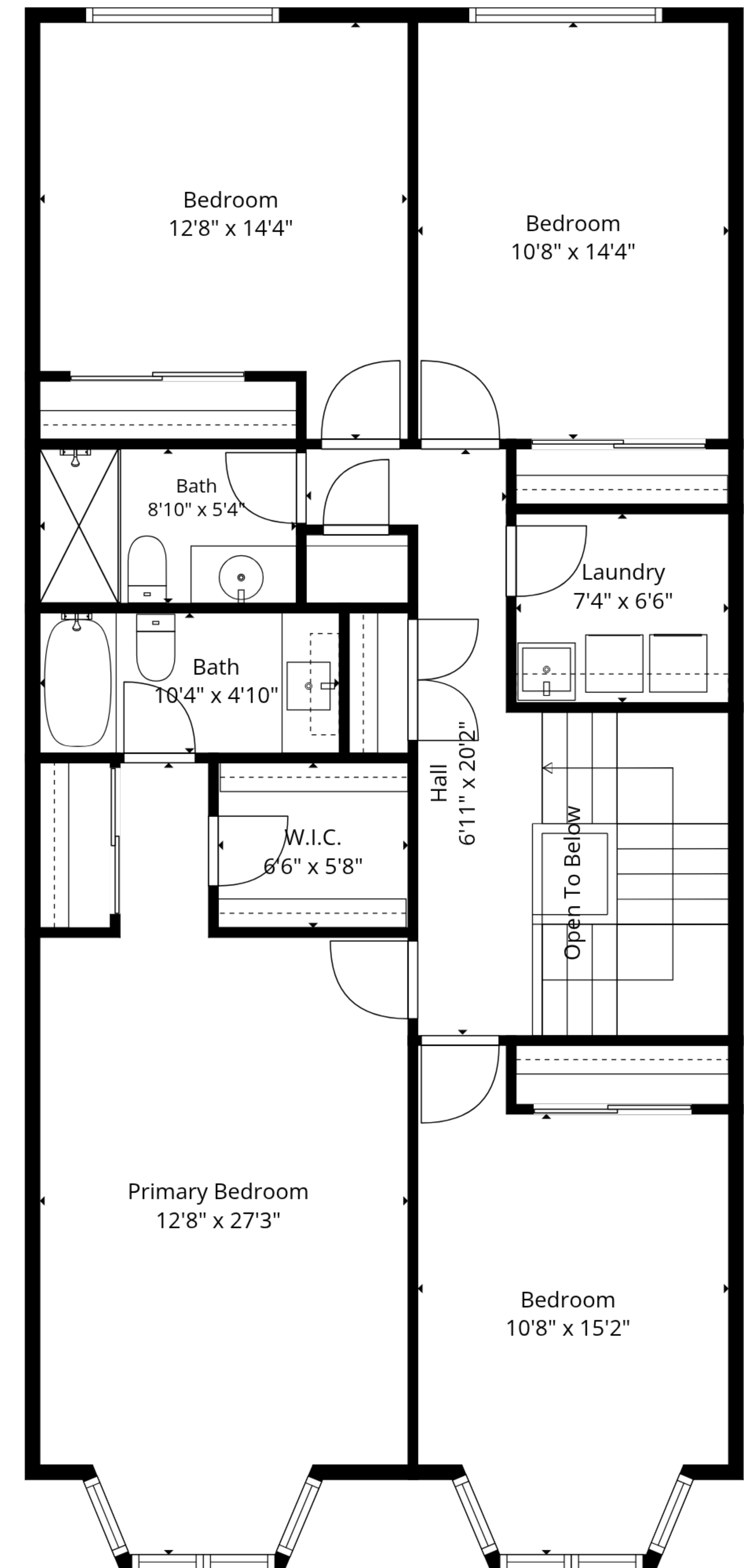
3rd Floor
