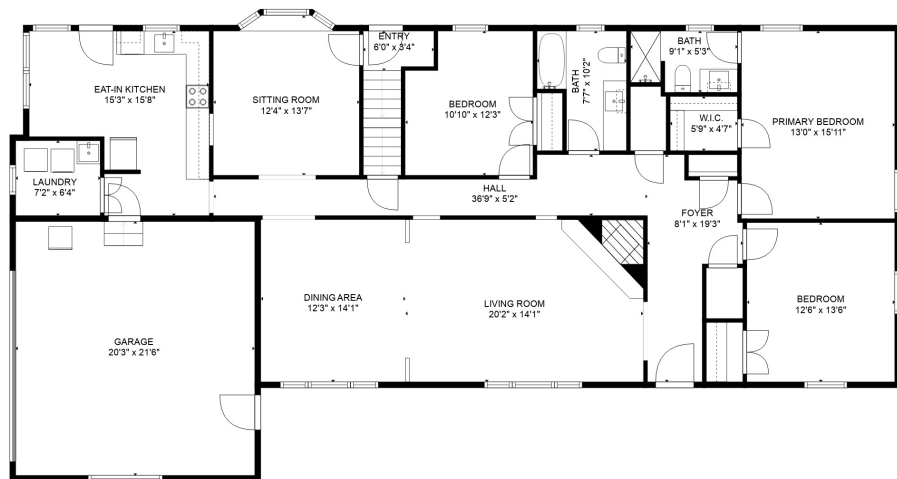
FLOOR 2
