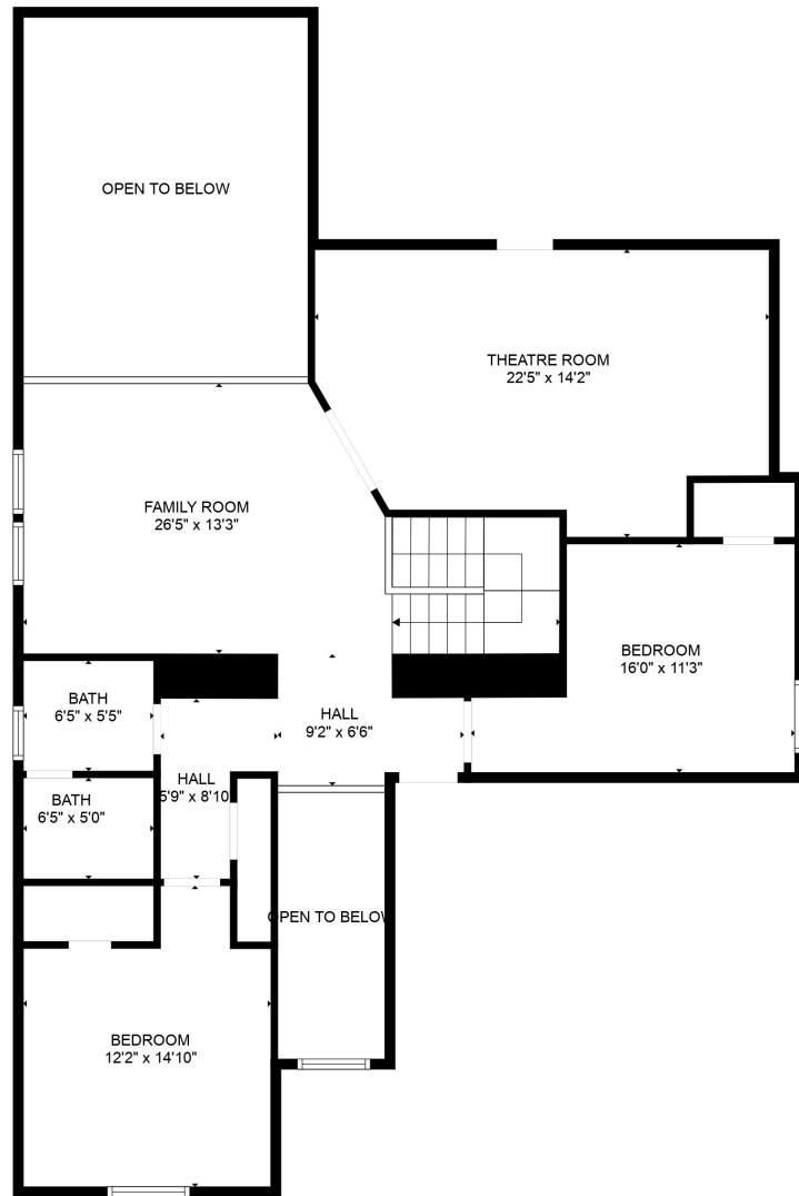
FLOOR 2
