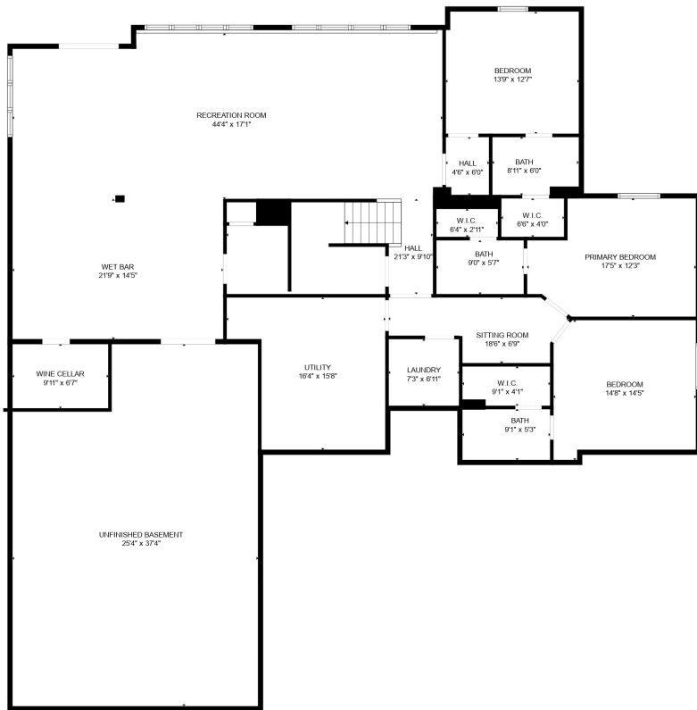
FLOOR 1
