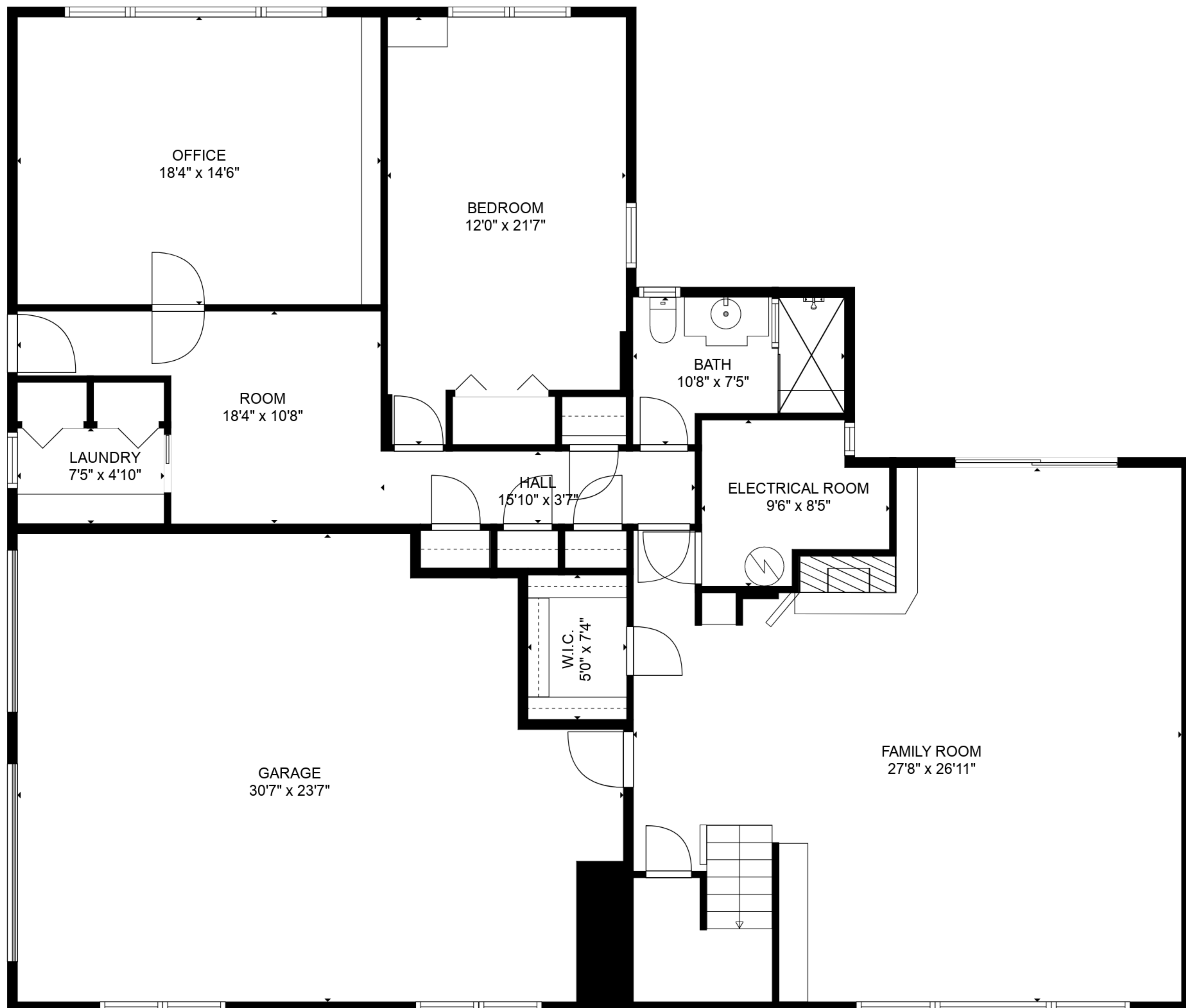
FLOOR 1
