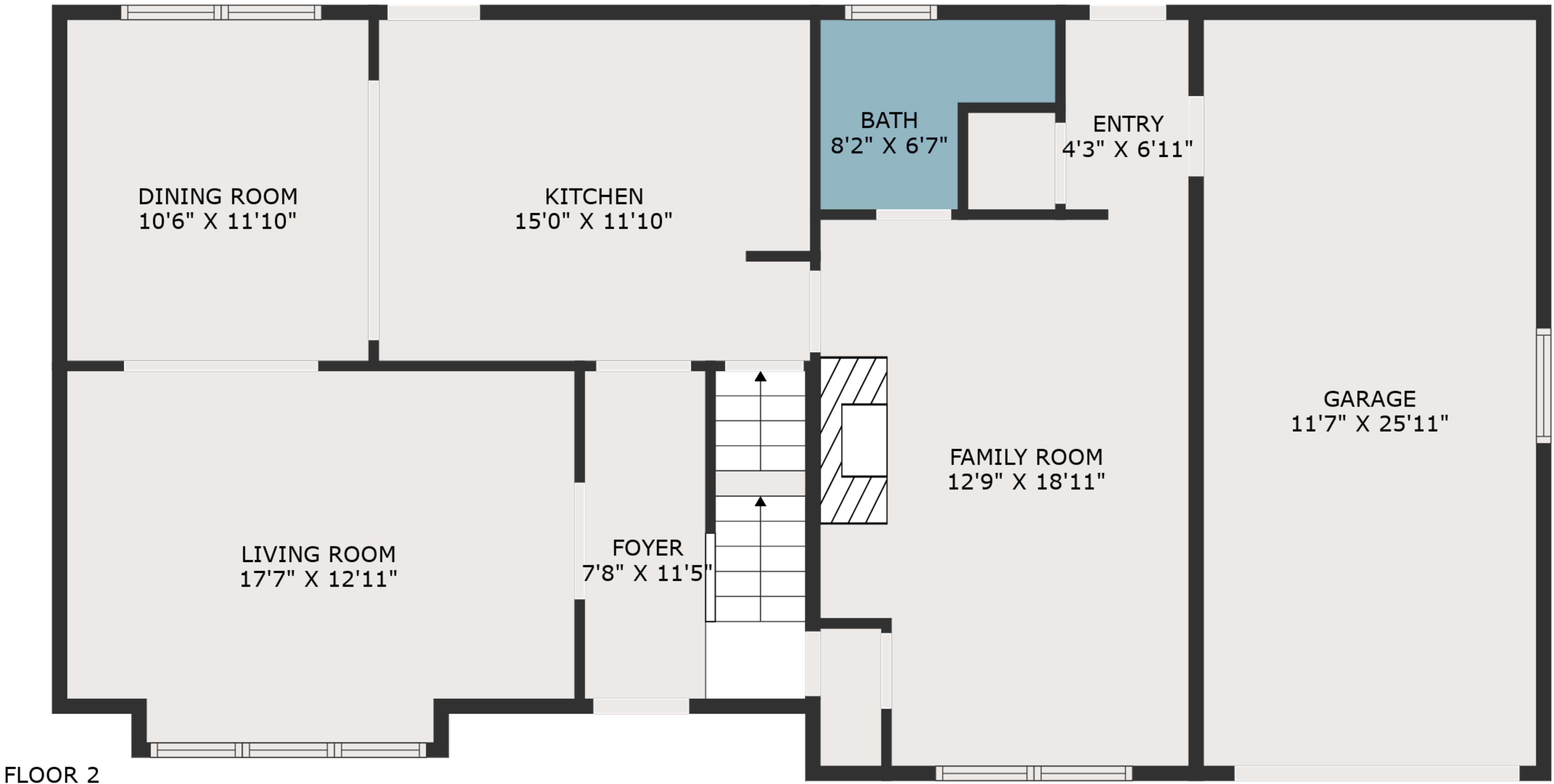
FLOOR 2
