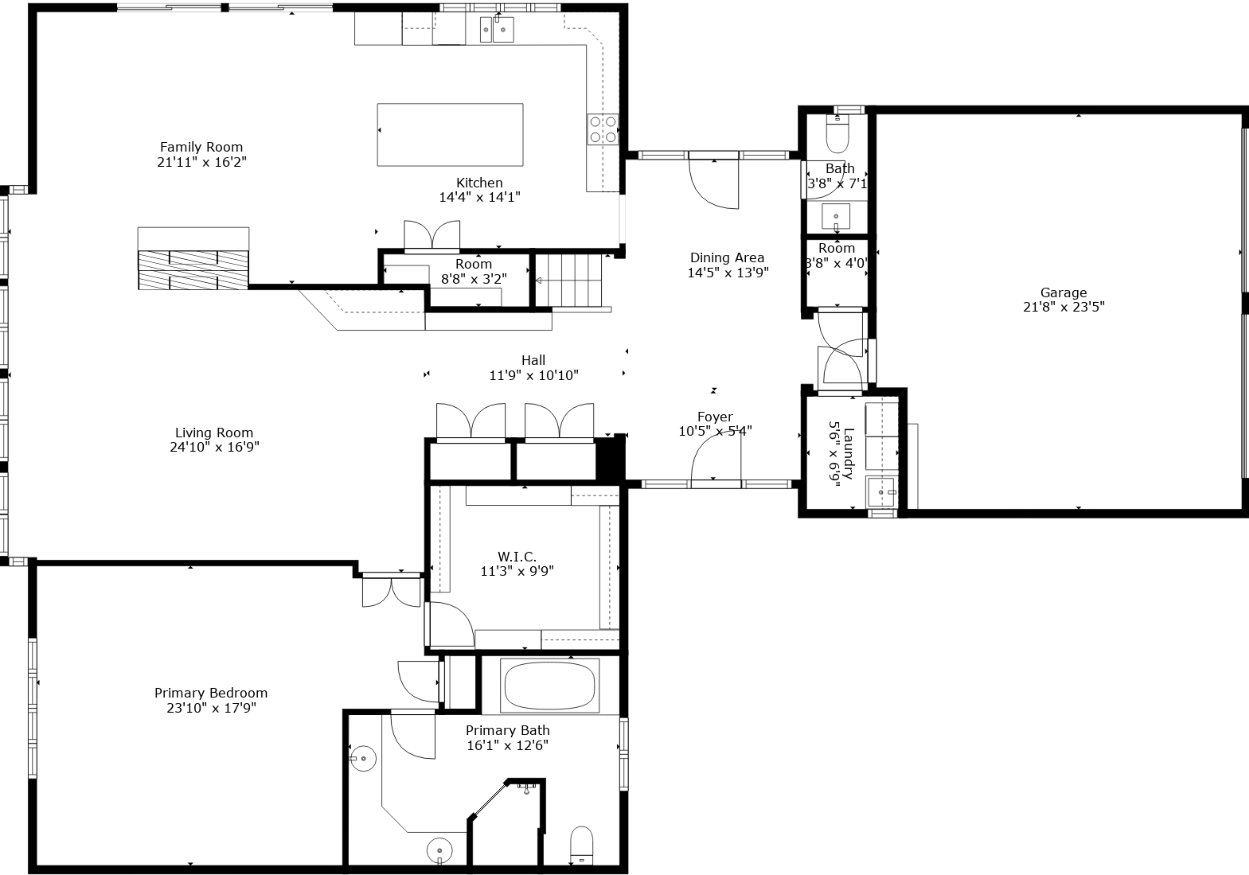
Floor 1
