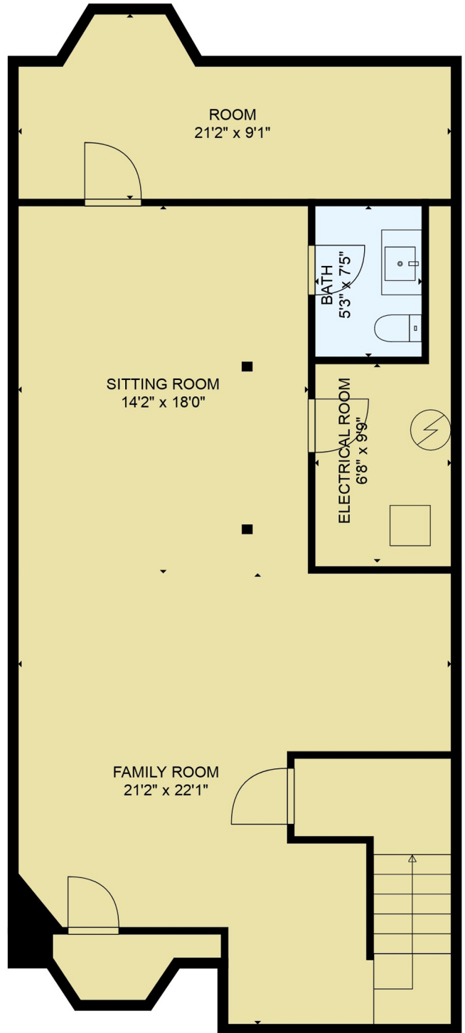
BASEMENT
