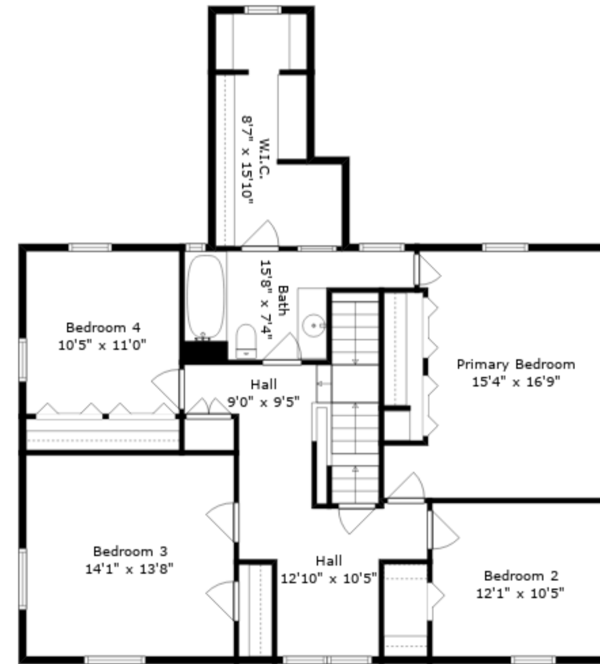
Upper Floor
