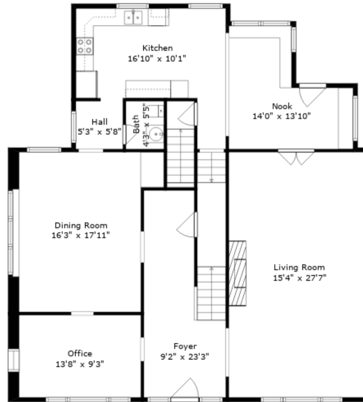
Main Floor
