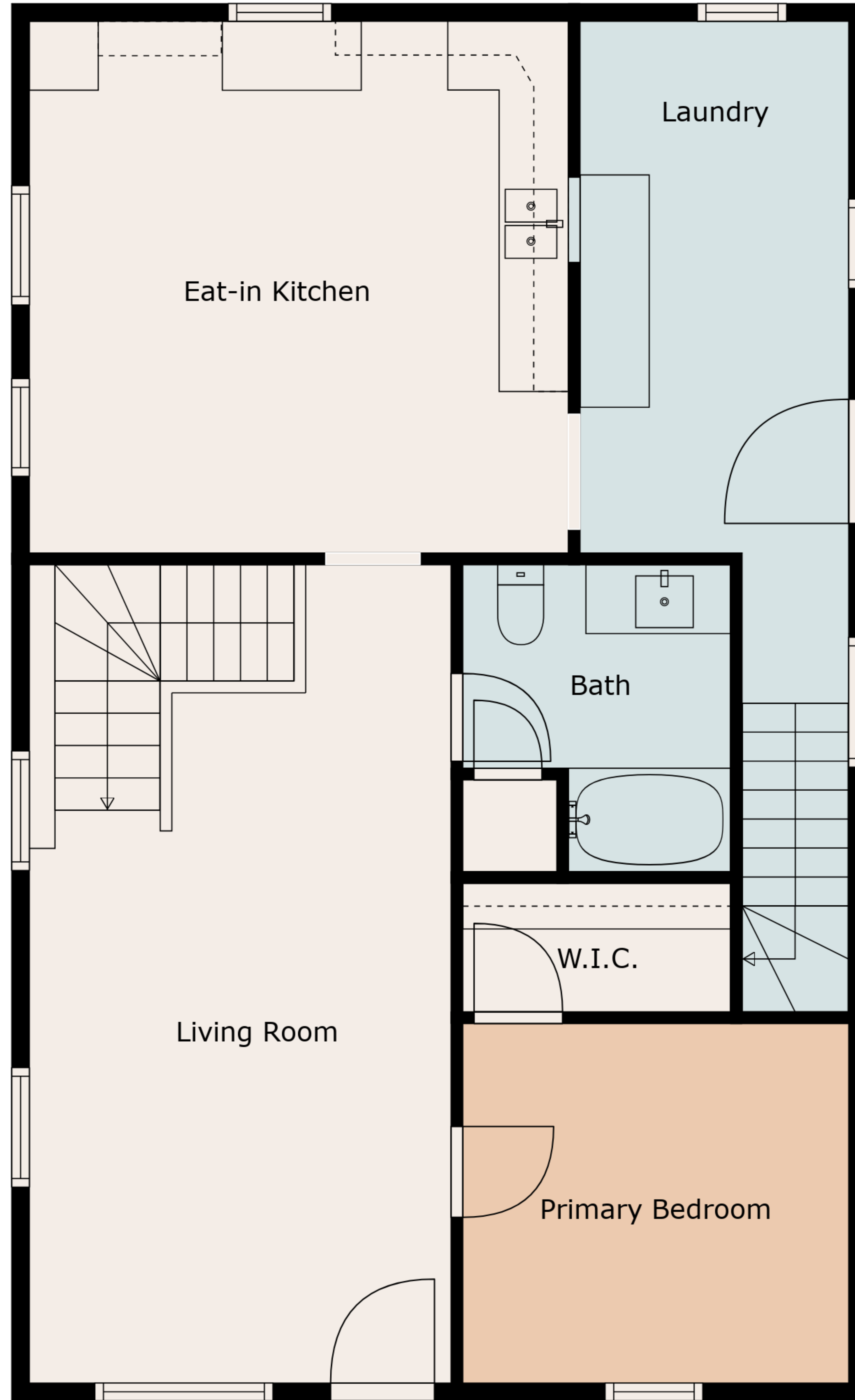
Floor 2
