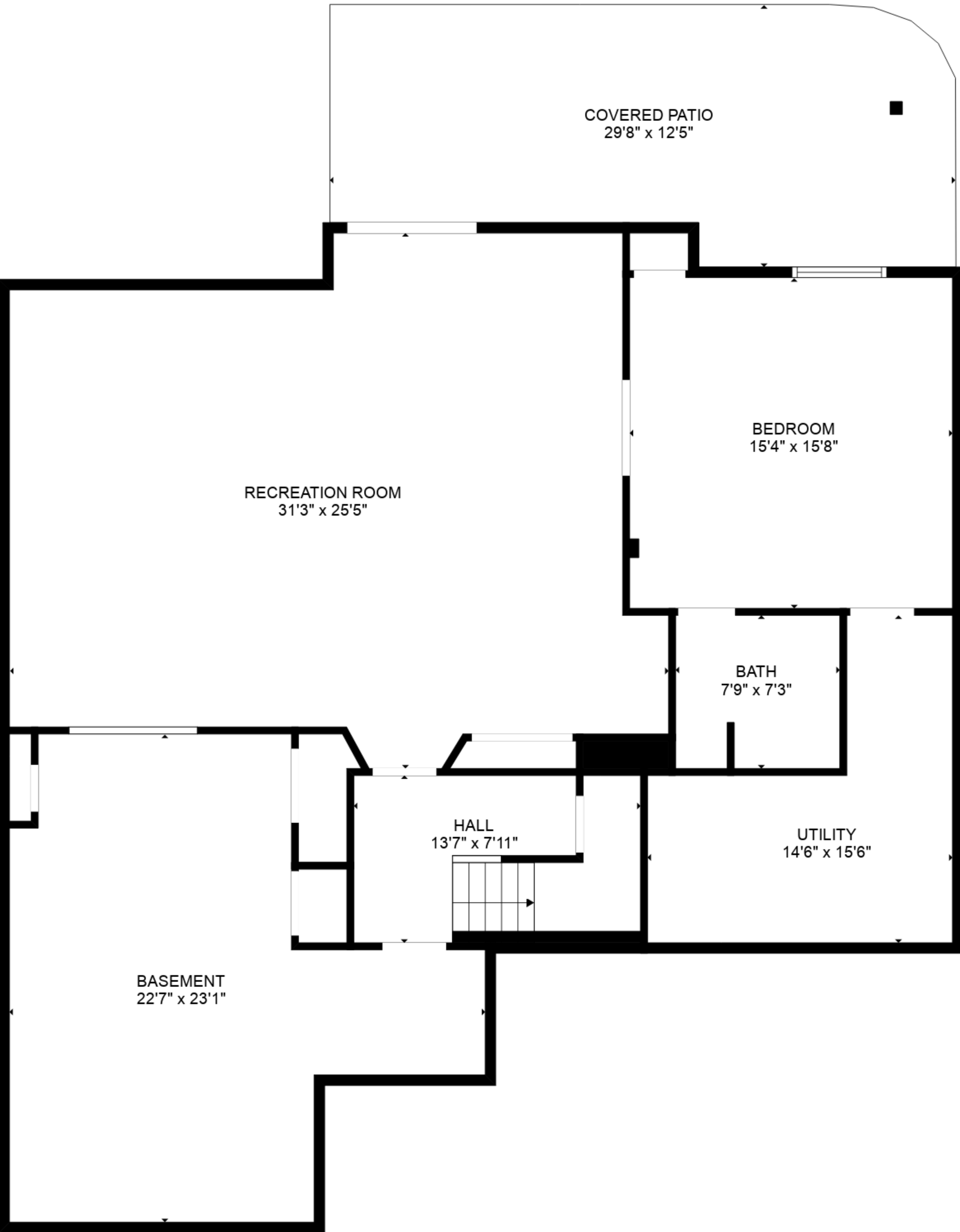
FLOOR 1
