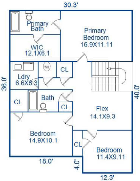
Second Floor 1140 sf
