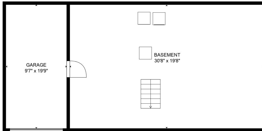
FLOOR 2
