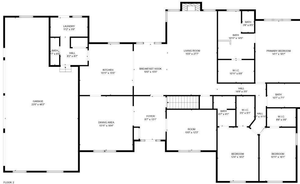
FLOOR 2
