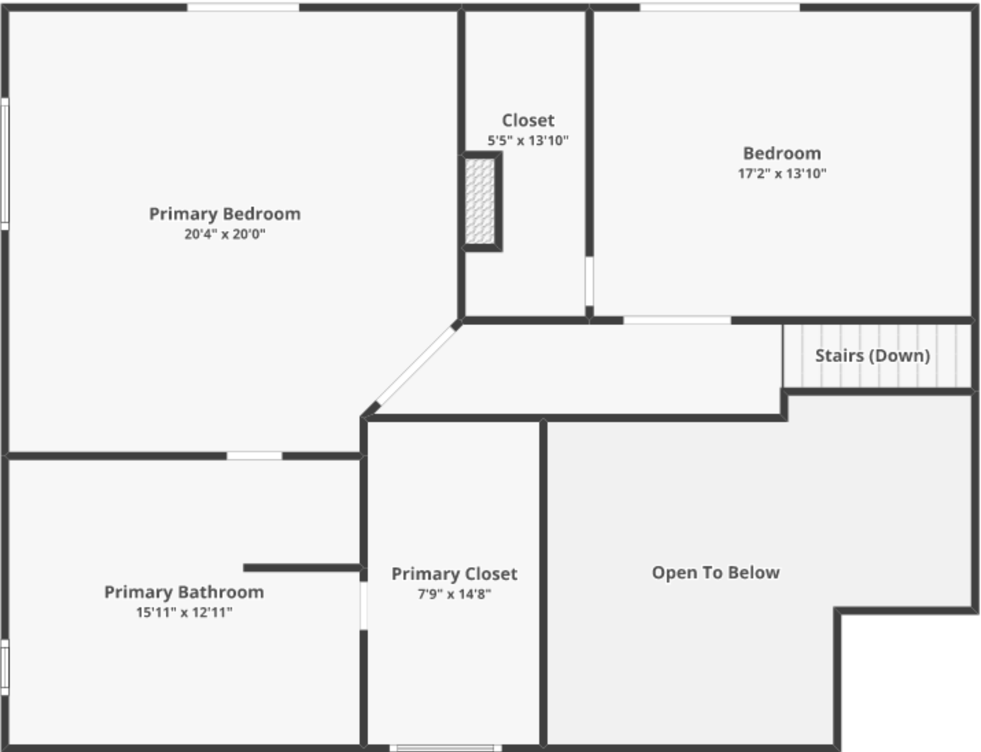
FLOOR 2
