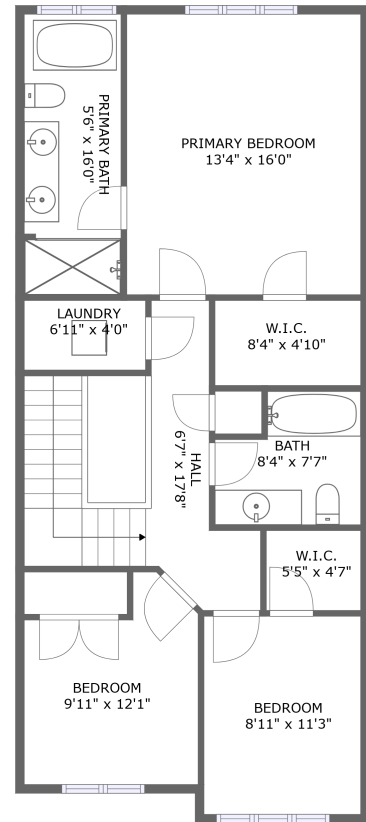
FLOOR 3
