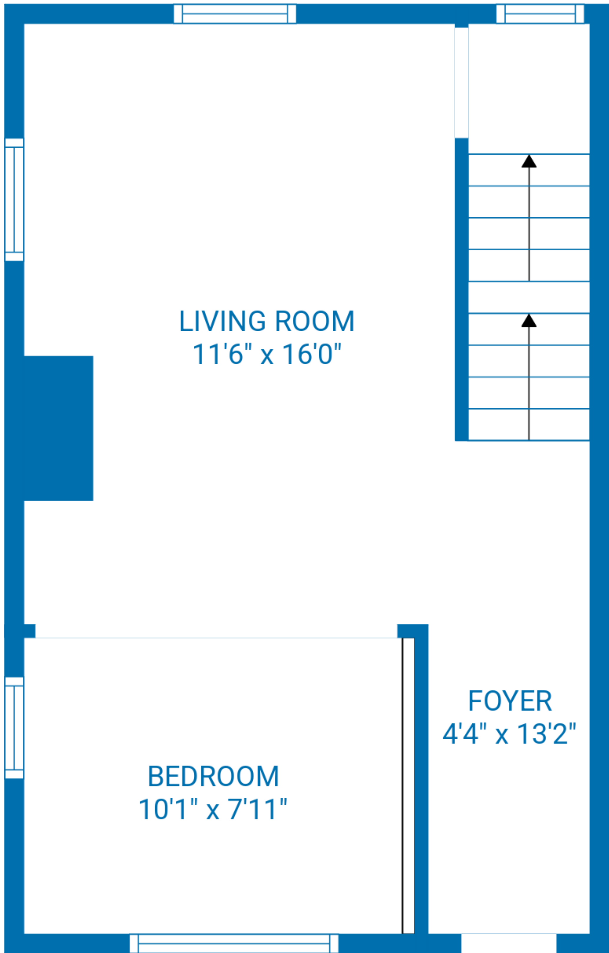
FLOOR 2
