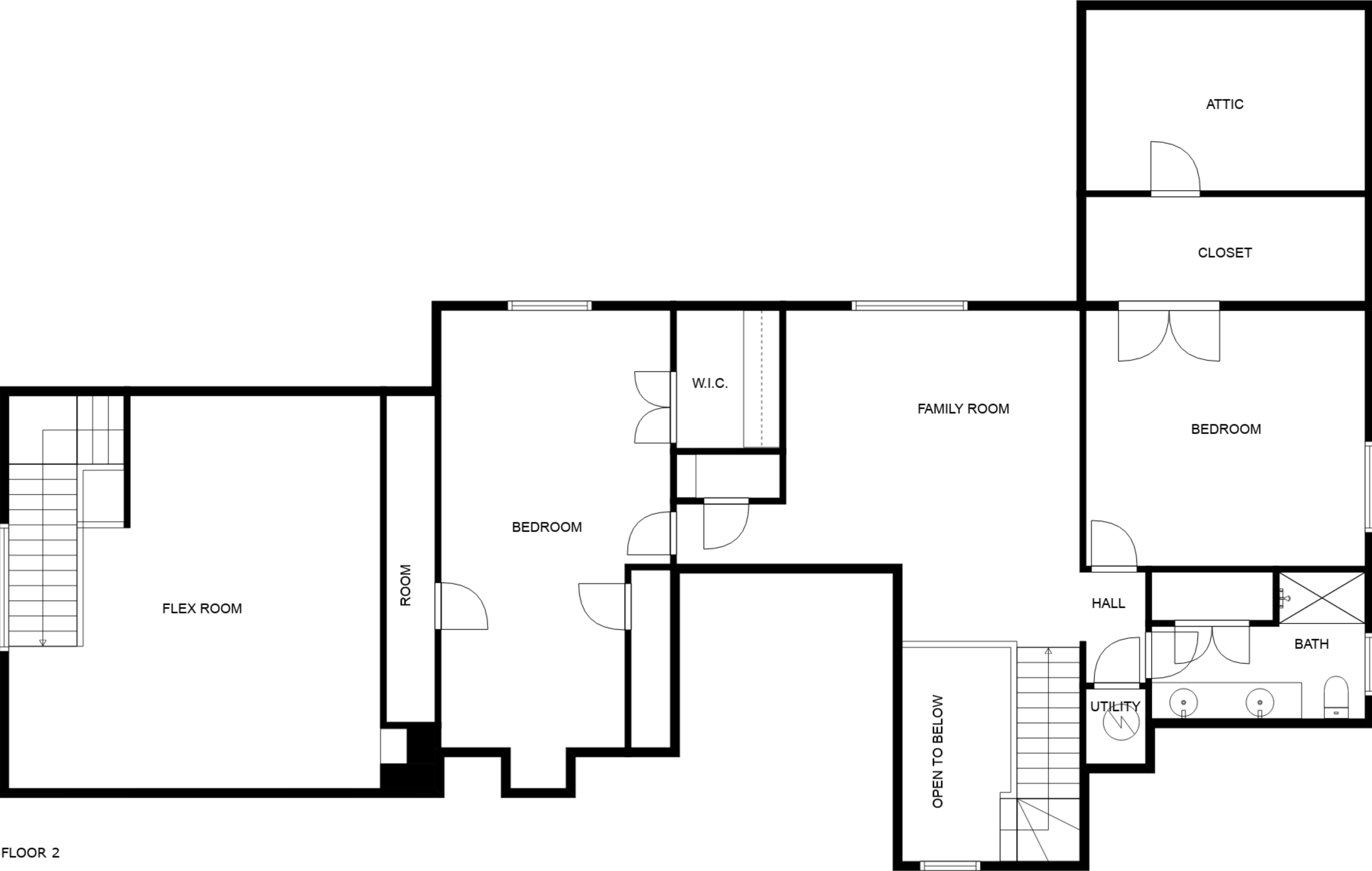
FLOOR 2
