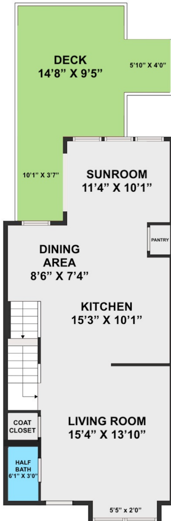
MAIN LEVEL 1947 LAUREL OAK DR.
