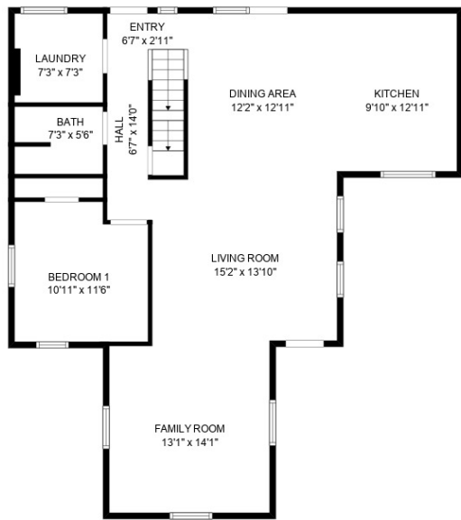
MAIN FLOOR
