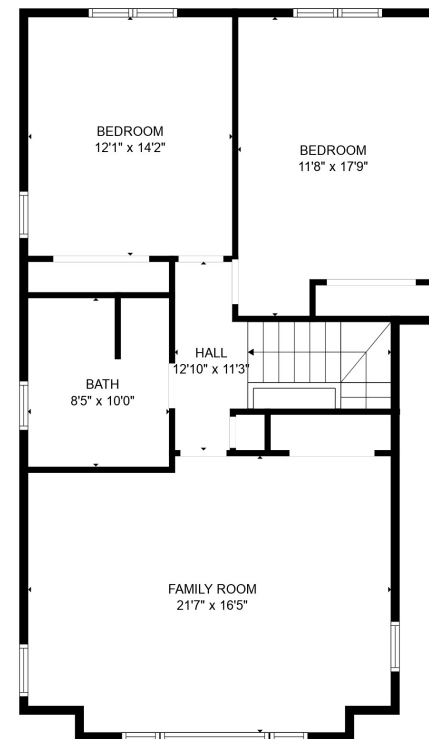
FLOOR 3
