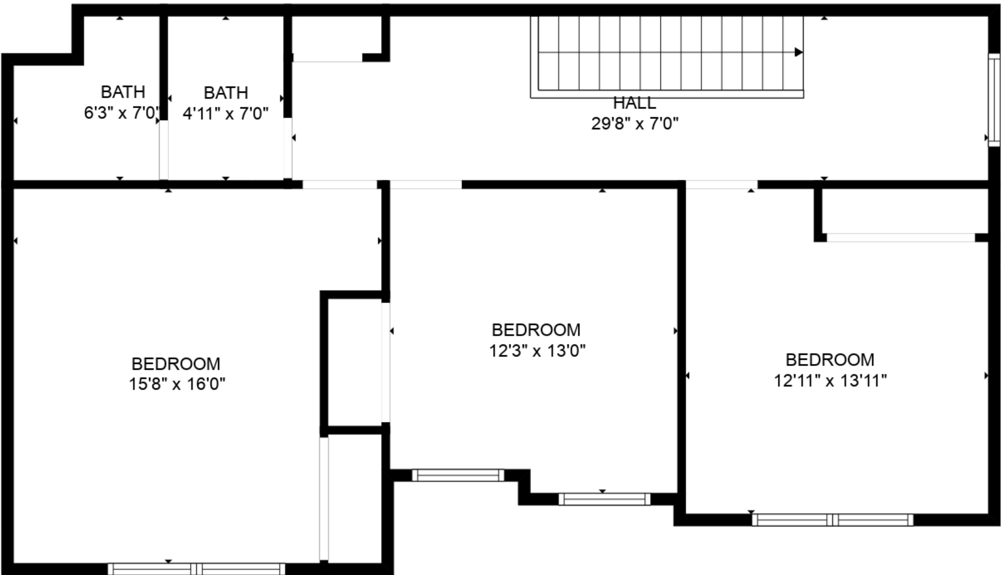
FLOOR 3
