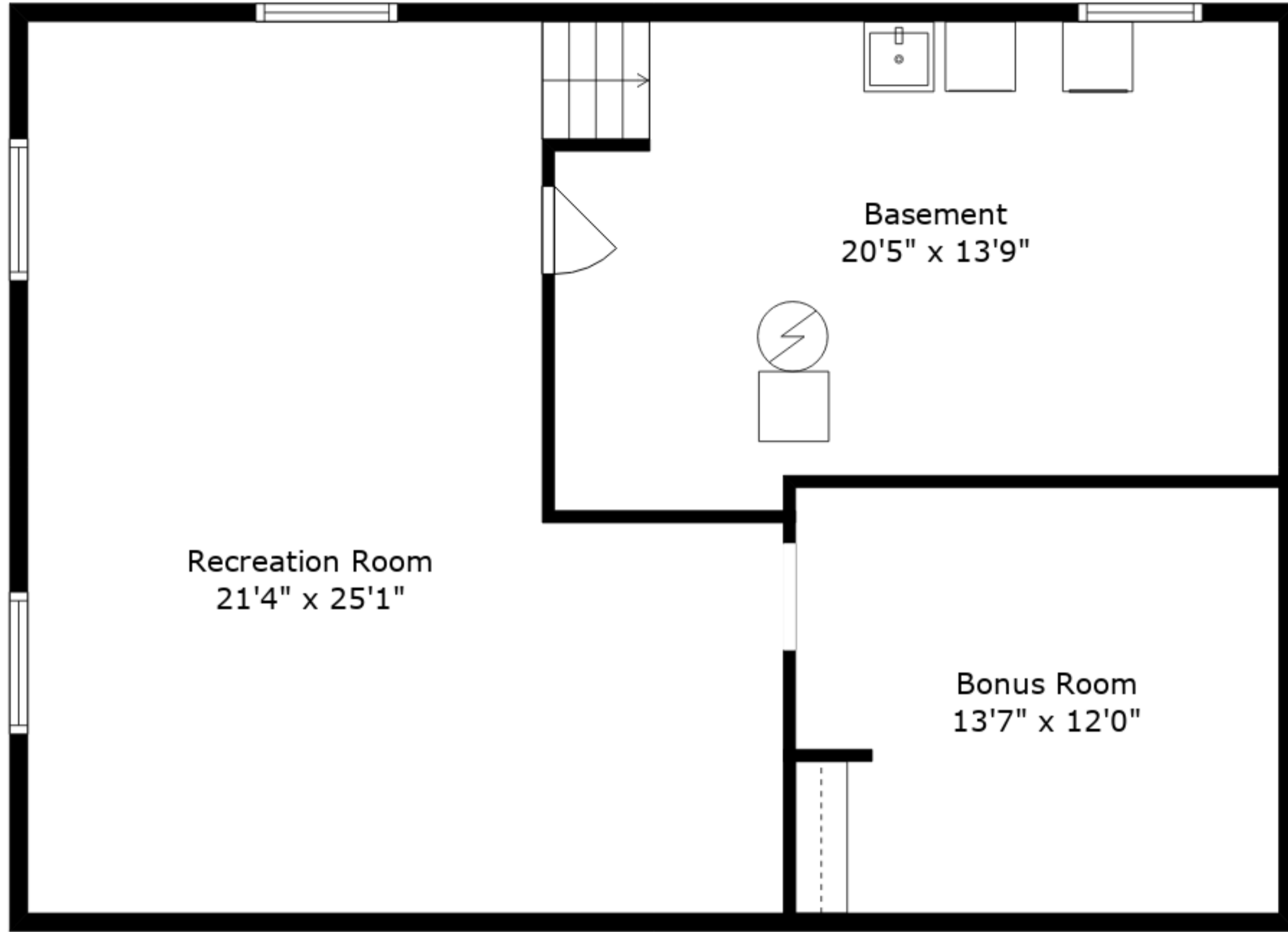
Lower Floor
