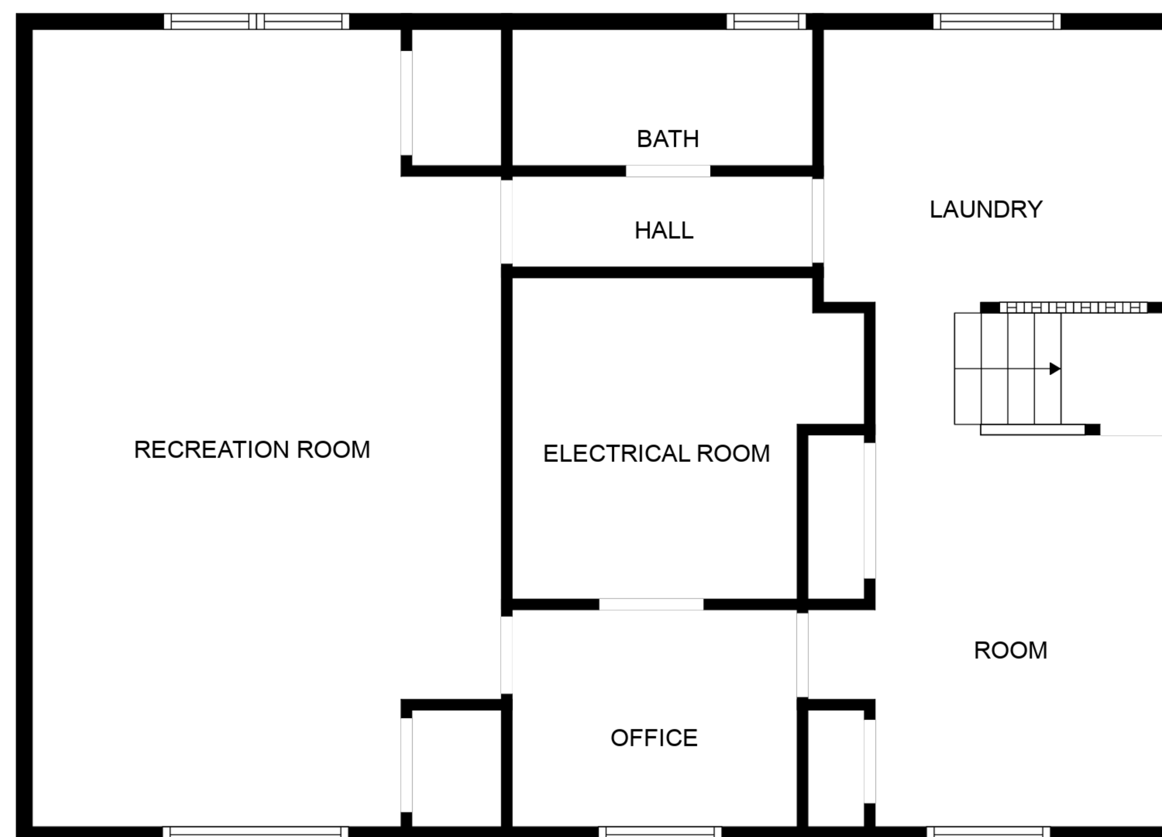
FLOOR 2
