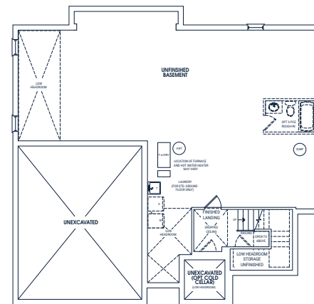
BASEMENT PLAN ELEVATION B
