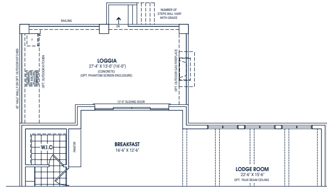
OPTIONAL GROUND FLOOR LOGGIA
