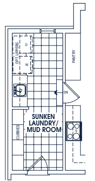
OPTIONAL GROUND FLOOR LAUNDRY/MUDROOM
