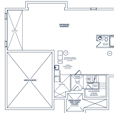
BASEMENT PLAN ELEVATION C
