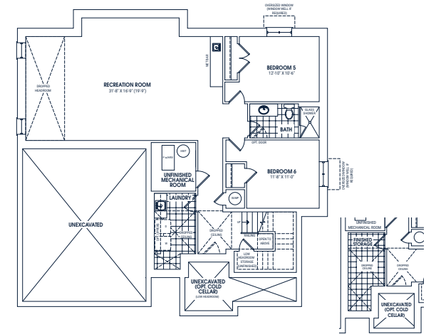
OPTIONAL FINISHED BASEMENT PLAN ELEVATION C
