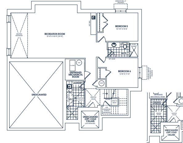
OPTIONAL FINISHED BASEMENT PLAN ELEVATION B
