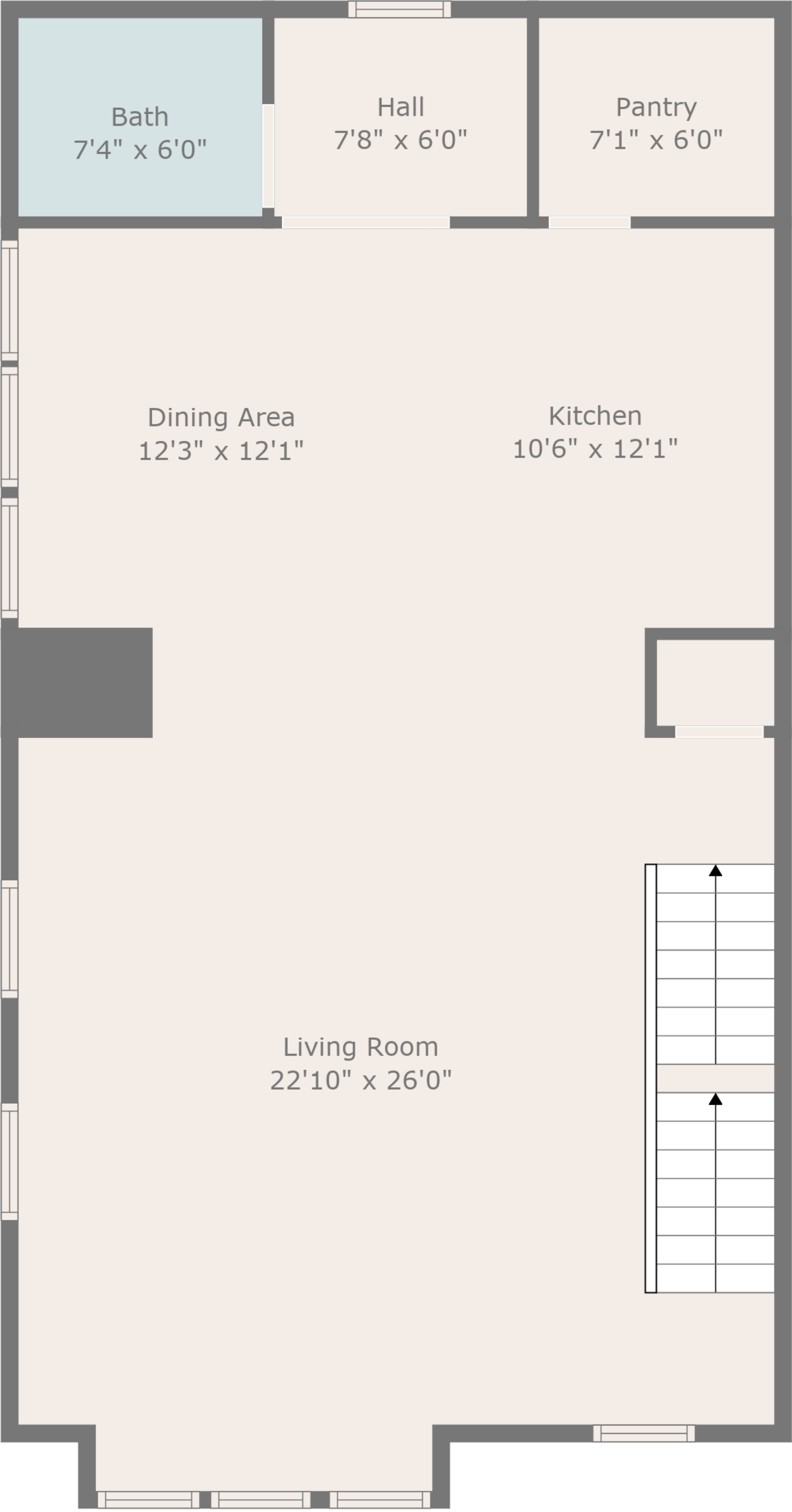
Floor 2
