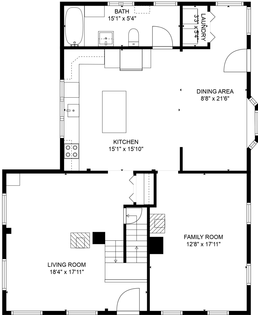
FLOOR 1
