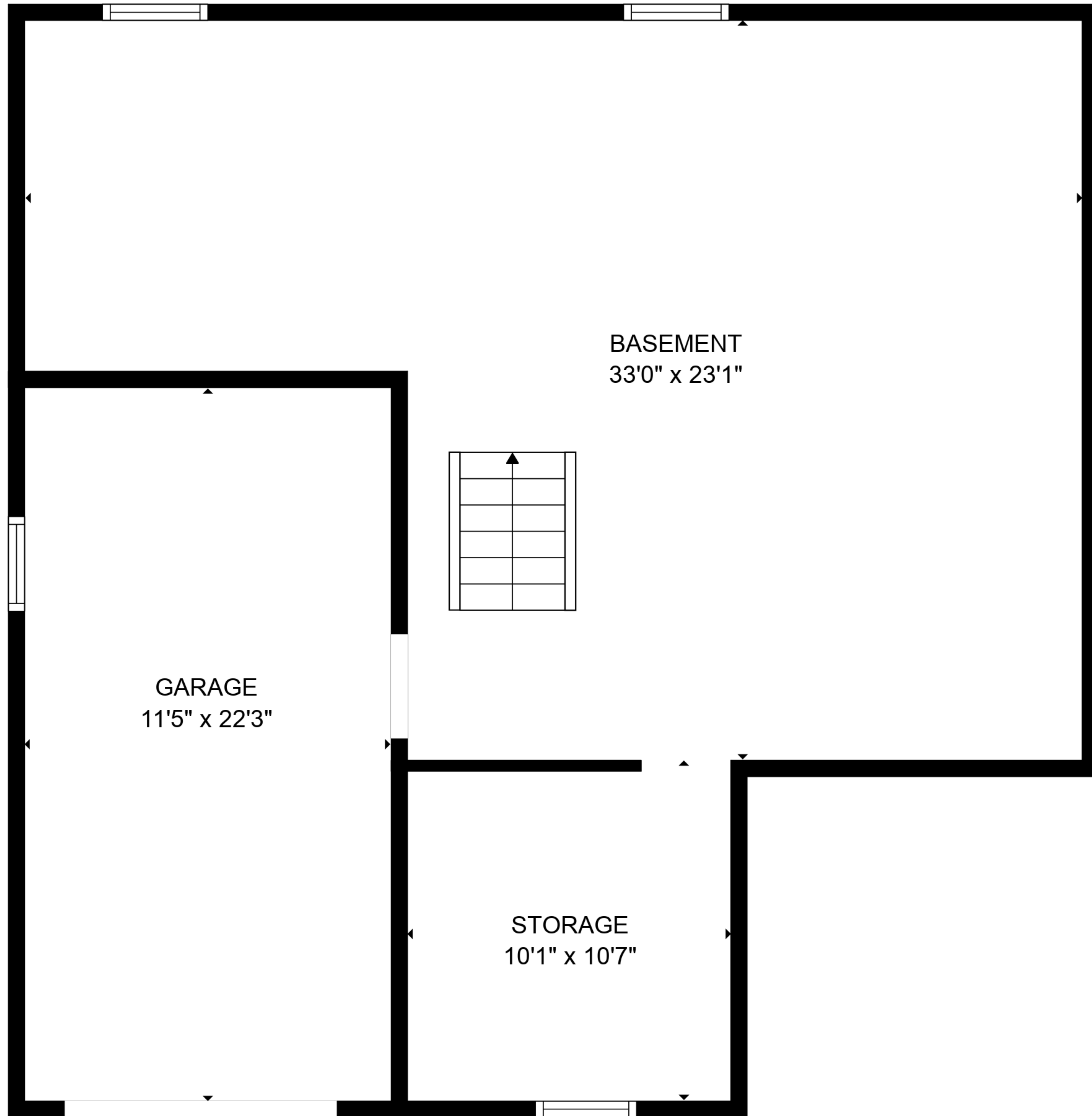
FLOOR 1
